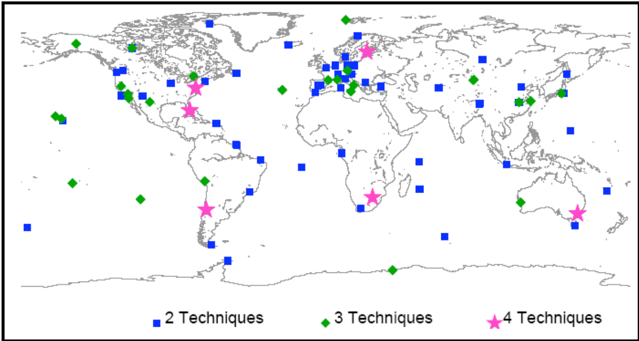
Figure 6. Current (from 2000) distribution of co-located space geodesy sites.
