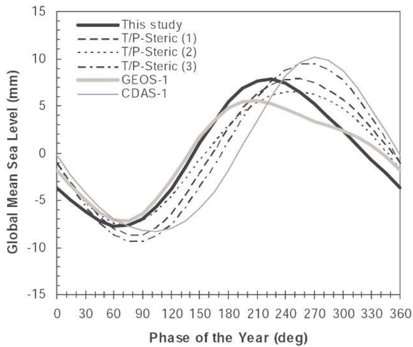
Figure 4. Global mean sea level determined through the theory of loading by GPS measurements of Earth's shape (This study) compared with direct measurements by Topex/Poseidon corrected for steric effects, and terrestrial hydrology, as inferred by mass conservation.
