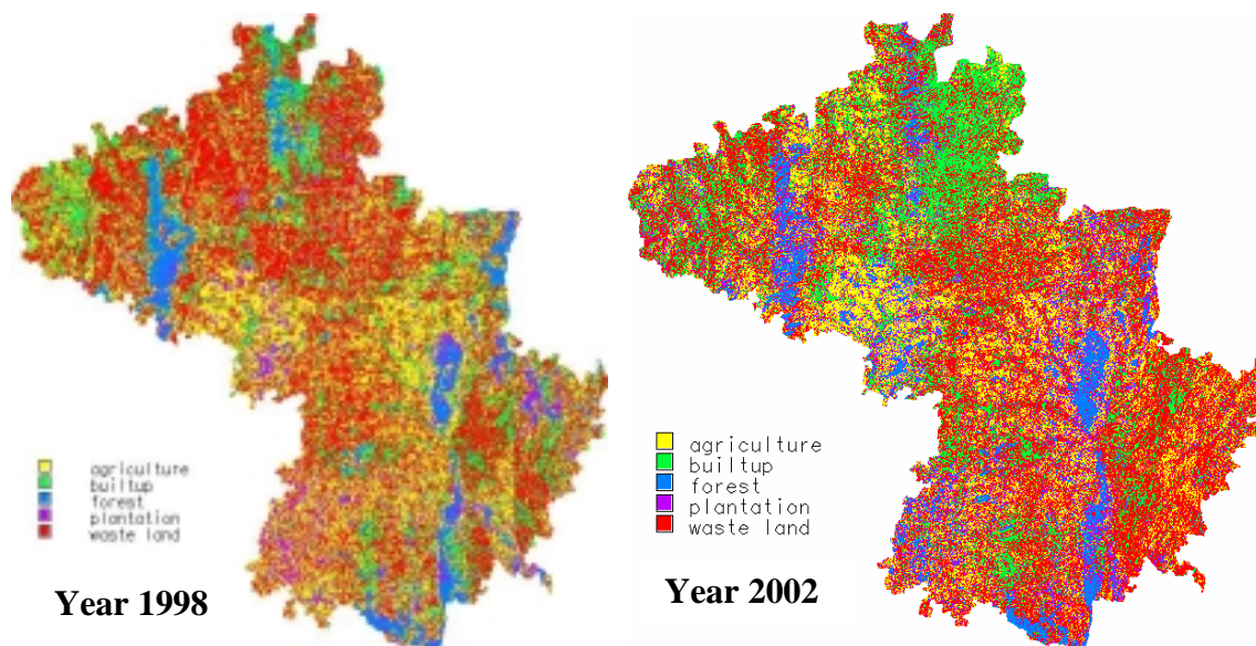
Figure4: Classified image
