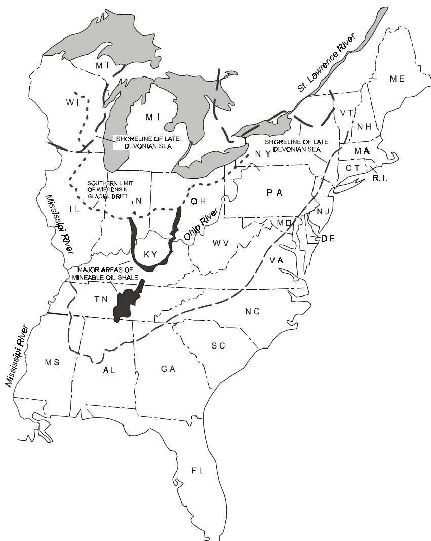
Fig. 17. Paleogeographic map showing shoreline of the late Devonian sea in eastern United States and major areas of surface-mineable Devonian oil shale. After Conant and Swanson (1961, Fig. 13) and Matthews and others (1980, Fig. 5)
