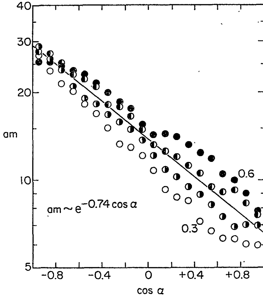
Figure 16. Reduced am as a function of \cos \alpha for f = 0.3 (open circles), f = 0.4 (circles open on the left), f = 0.5 (circles filled on the left), and f = 0.6 (filled circles). The scale for am is logarithmic. An expression of the form am = k \exp(-g \cos \alpha) fits the data.
