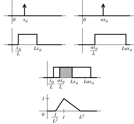
Figure 2: Top Row: A signal of a single impulse and a dilated version of the same signal, Second Row: The geometric blur of each signal, Third Row: Overlay of the two signals after geometric blur. The shaded region contributes to the correlation at zero offset. Fourth Row: Relative overlap as a function of dilation.
