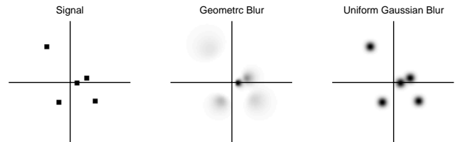
Figure 4: Geometric Blur with a spatially varying Gaussian kernel blurs more farther from the origin.
