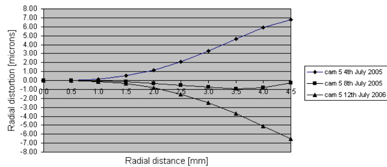
FIG. 9. Radial distortion curves showing differences with respect to a mean curve for camera five and three sets of IOP
