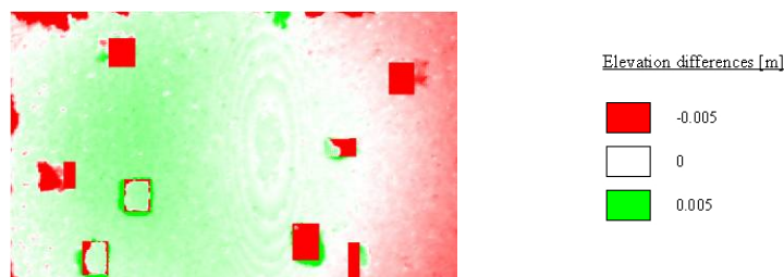
FIG. 8. Difference image with base to distance ratio of 1:2
