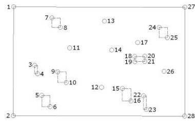
FIG. 3. Position of photogrammetric target points.
