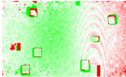
FIG. 5. Elevation differences-IOP: 4 th July 2005.
