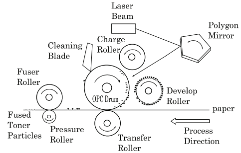
Fig. 2. EP printing process overview
