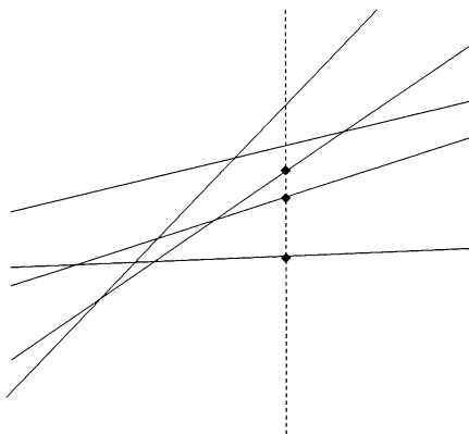
Fig. 1. Minimum weight base in a uniform matroid with positive-slope weight functions.
