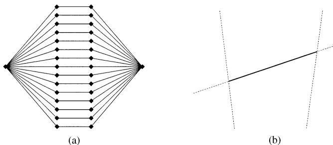
Fig. 3. Lower bound construction for graphic matroids: (a) the graph G ; (b) weight functions for the three edges corresponding to a line segment.
