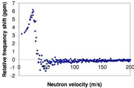
FIG. 15. (Color online) Results of computer simulations for the shift in the ratio |(\omega_{L_n}/\omega_{L_{Hg}})| with varying neutron velocity, when there is a gradient \partial B_{0z}/\partial z = 20 \text{ nT/m} in a \mathbf{B}_0 field of 1 \mu\text{T} . The shifts are caused by the different averaging, for the two species, of the B_x and B_y field components that must accompany this gradient. The shift at zero velocity is consistent with Eq. (89). When the neutrons travel as fast as the Hg atoms the shift becomes zero.
