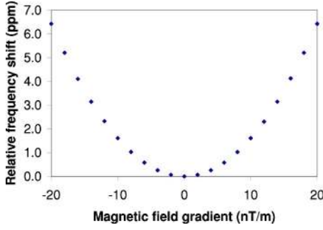
FIG. 14. (Color online) Results of computer simulations for the shift in the ratio |(\omega_{L_n}/\omega_{L_{Hg}})| with varying gradients q in a small \mathbf{B} field, B_z=0 , B_x=qy , B_y=qx , when it is added to a uniform \mathbf{B}_0 field of 1 \mu\text{T} aligned with the z axis. The shift is caused by the different averaging of B_x and B_y by the two species. These results are consistent with Eq. (88).
