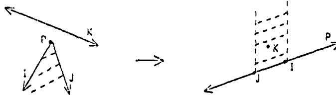
Figure 3-4: Transform of a redundant half-plane.
