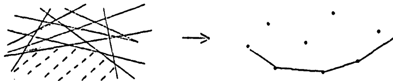
Figure 3-5: Transform of N UPPER half-planes.
