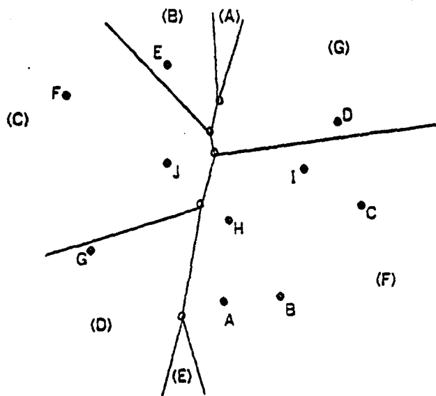
Figure 4-1: Planar Nearest Point Voronoi Diagram
