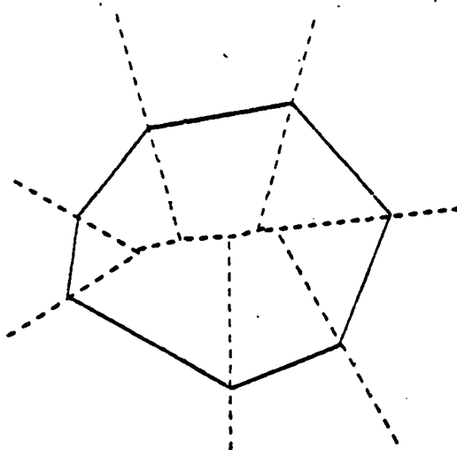
Figure 4-6: Nearest edge diagram of a convex polygon.
