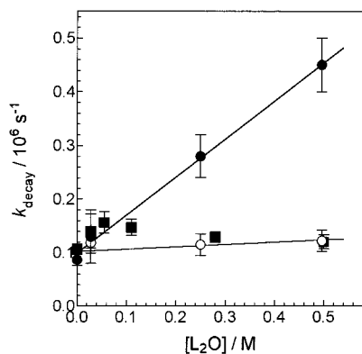
Figure 3. Plot of k_{\text{decay}} vs [\text{L}_2\text{O}] concentration for ketones 7a (●, \text{H}_2\text{O} ; ○, \text{D}_2\text{O} ) and 7b (■, \text{H}_2\text{O} ) in deoxygenated acetonitrile solution. k_{\text{decay}} values for 7a were obtained from the intercepts of dilution plots at each [\text{L}_2\text{O}] concentration.
