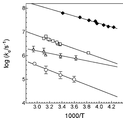
Figure 4. Arrhenius plots of the triplet decay rates (at infinite dilution) of phenolic ketones 1 (◆), 5a (□), 6a (△), and 7a (○) in deoxygenated acetonitrile solution.
