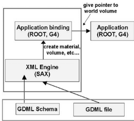
Fig. 3. GDML reader.
