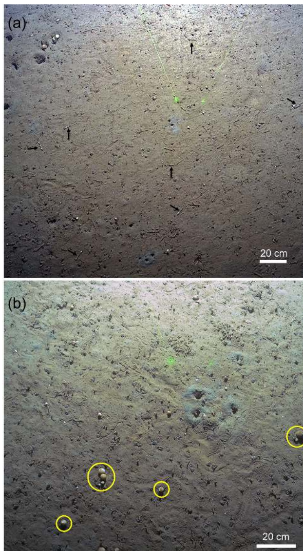
Figure 8. (a) Examples of the onuphid worm, Nothria conchylega (a few individuals are highlighted with black arrows). Note trails in the sediment behind the onuphids, indicating they crawl on the seafloor surface. (b) Examples of Thenaea sponges (possibly Thenaea valdiviae ). A few individuals are circled in yellow.
