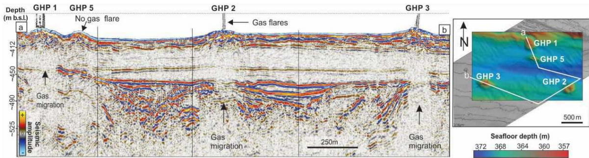
Figure 6. Seismic profile of the four study pings. The transect for the seismic profile is shown in the map of the study site, starting near GHP1 (point a) and ending near GHP3 (point b). Zones of acoustic blanking beneath the three free-gas-emitting pings are highlighted with arrows. This kind of blanking was not seen below GHP5.
