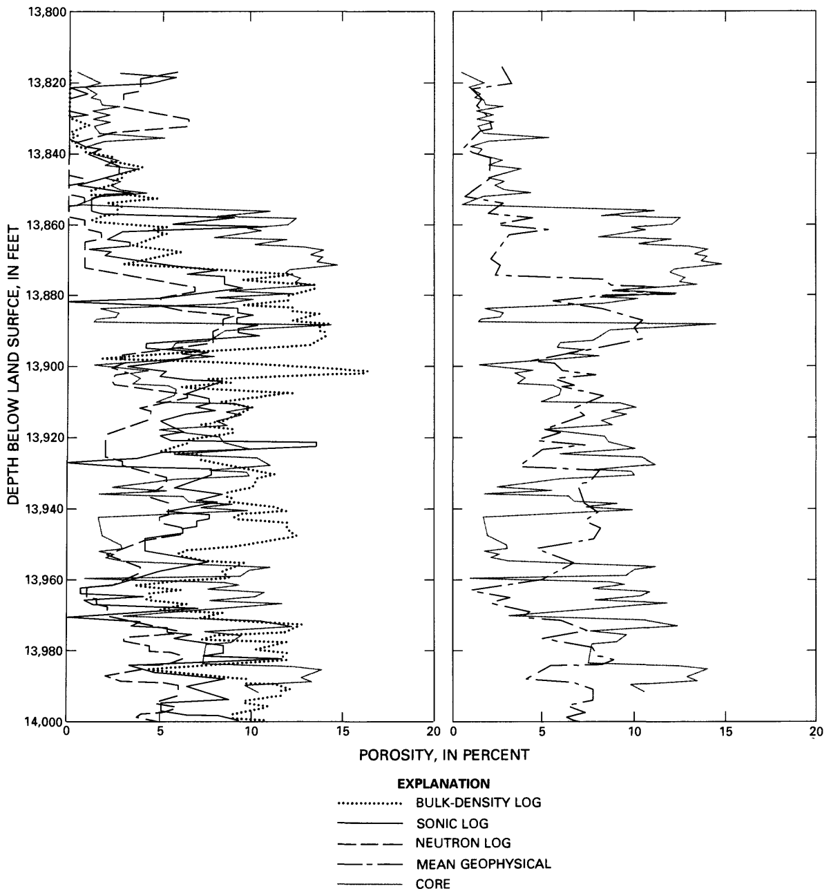
Figure 11.--Comparison of porosity values estimated by geophysical methods and by laboratory core analysis for the Tensleep Sandstone in borehole 21.
