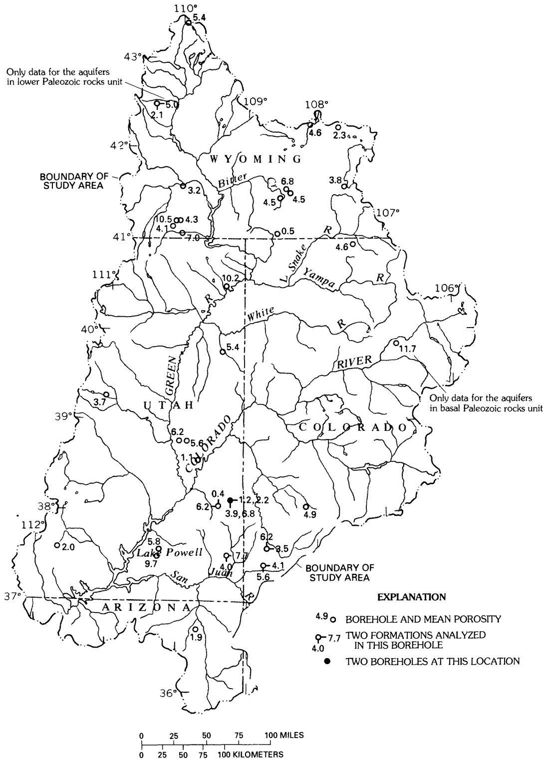
Figure 16.--Grand mean geophysically estimated porosity of aquifers in the middle, lower, and basal Paleozoic rocks.
