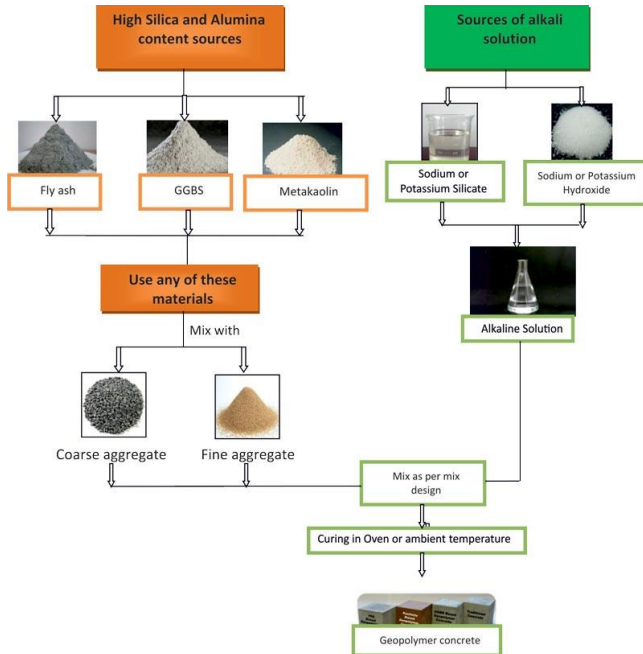
Fig. Production of Geopolymer Concrete [1]
