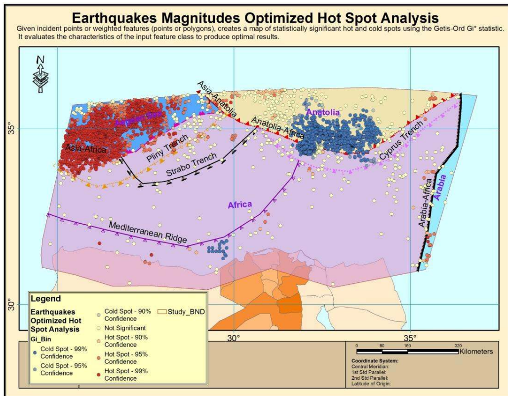
Fig. 5. Spatial statistical mapping of the earthquakes' magnitudes by Hot Spot Analysis (Gets-Ord Gi*)
