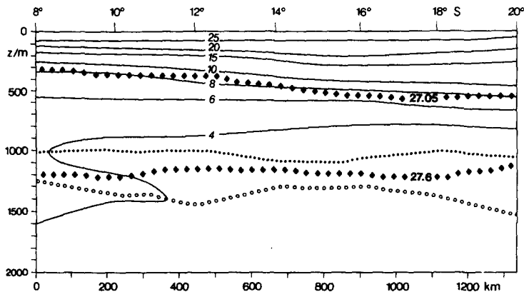
Fig. 3. Vertical distribution of temperature in °C in the upper 2000 m along the north (left)–south (right) line of stations occupied by Prof. Vize at 30°W in April 1969. Relative minima are denoted by dots and maxima by open circles. Also shown are the isopycnals of \sigma_\theta = 27.05 and 27.6 \text{ kg m}^{-3} (diamonds).
