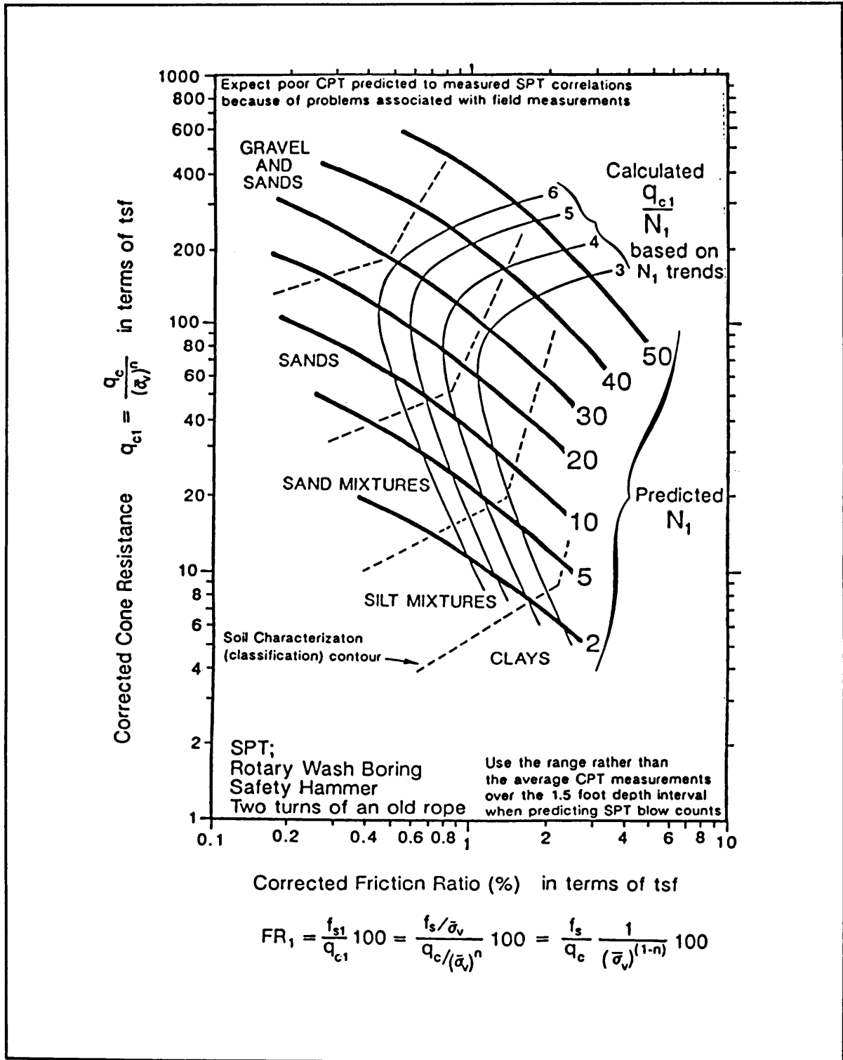
Figure 28. Correlation of CPT and SPT data (After Olsen and Malone 1988)
