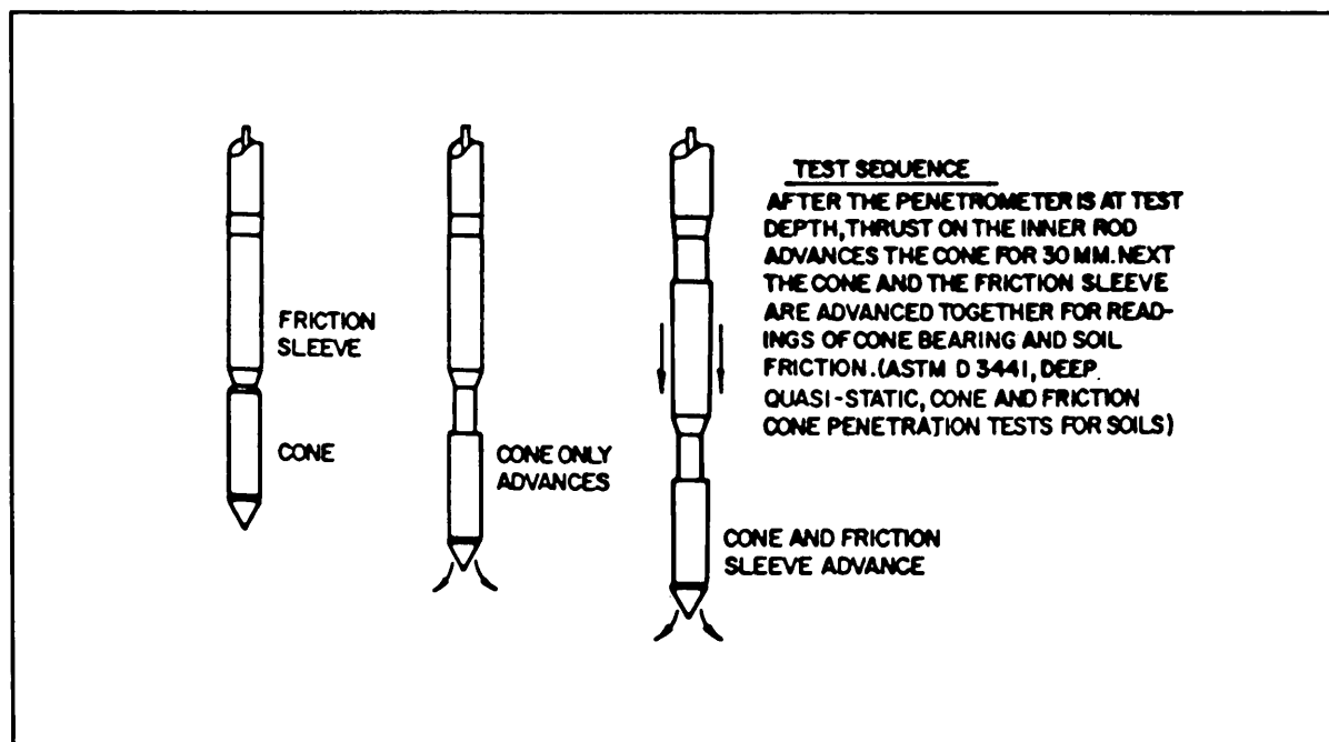
Figure 25. Cone penetrometer tip and sleeve
