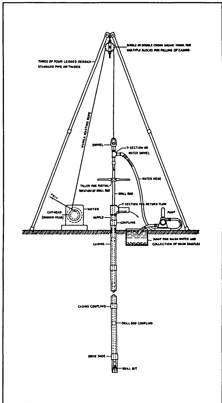
Figure 19. Wash boring system
