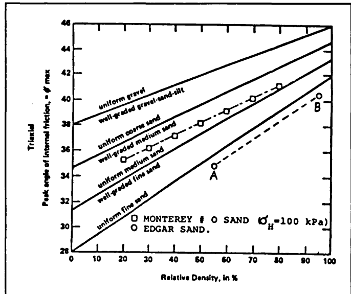
Figure 9. Effect of relative density on friction angle for sands
