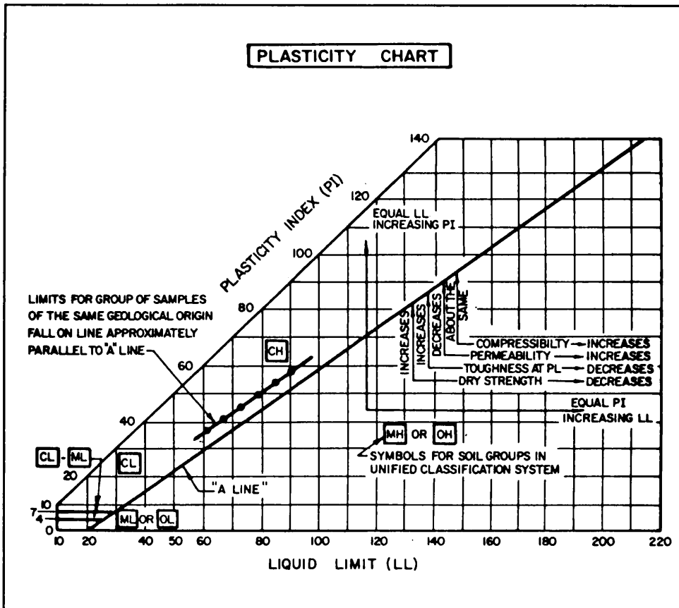
Figure 2. Casagrande plasticity chart for cohesive soils (NAVFAC 1982)
