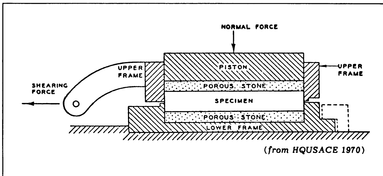
Figure 5. Schematic diagram of direct shear box
