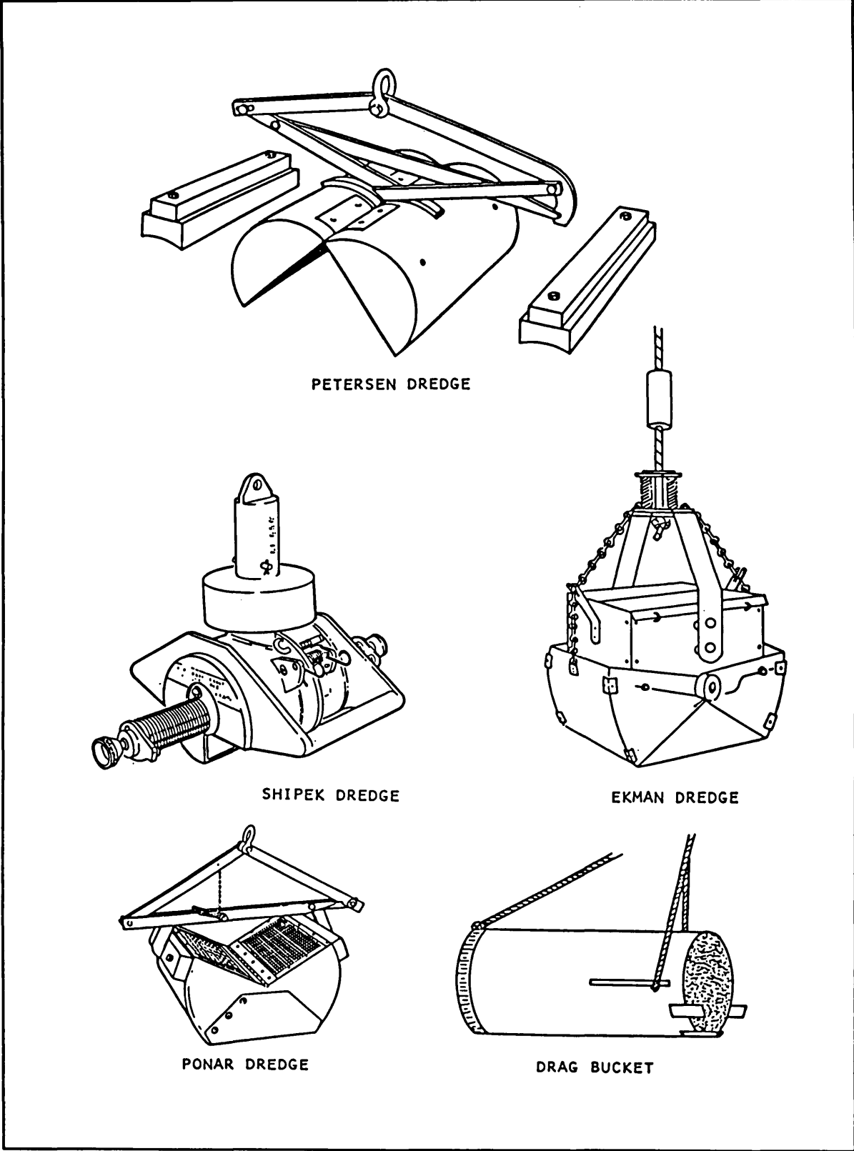
Figure 18. Various designs of surface soil samplers
