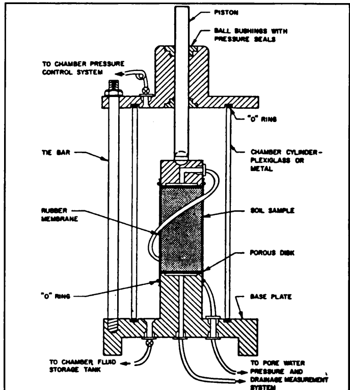
Figure 7. Schematic diagram of triaxial compression apparatus
