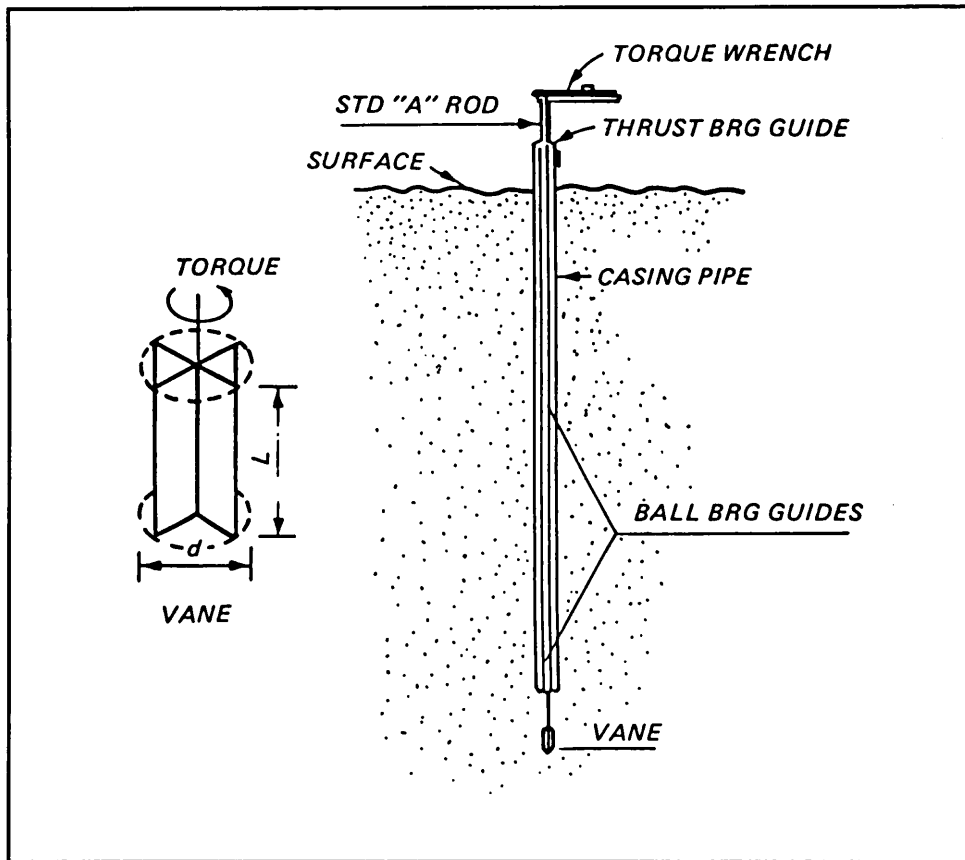
Figure 23. Field vane shear test
