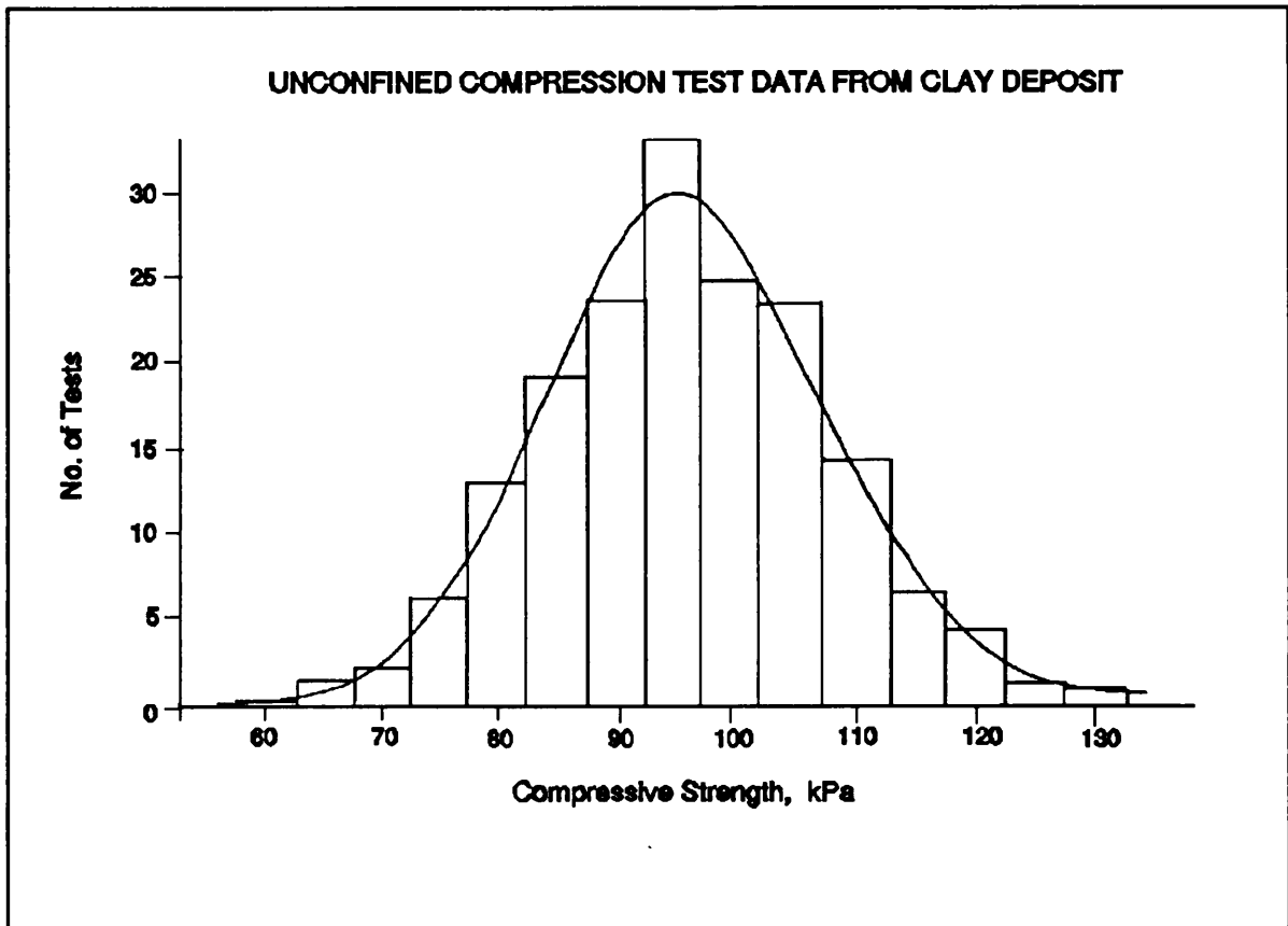
Figure 30. Frequency histogram of soil property test data
