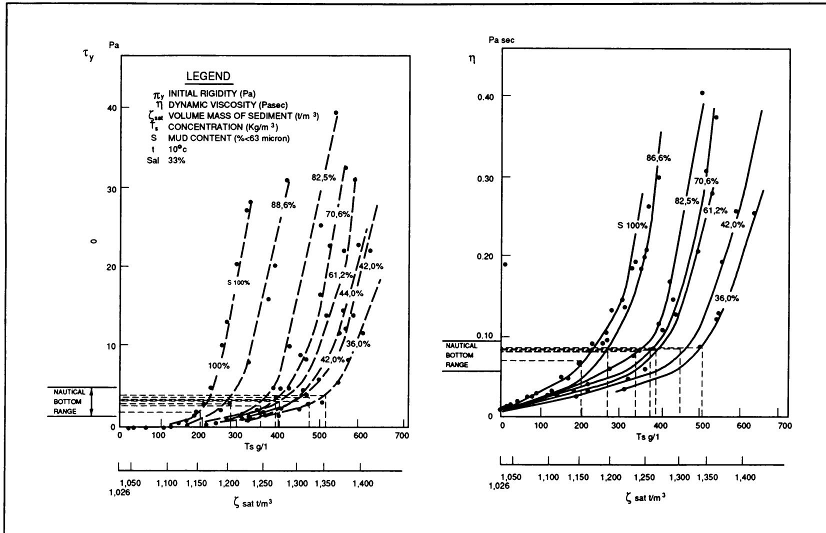
Figure 12. Relationship between yield stress and viscosity and slurry density (Meyer and Mahlherbe 1987)
