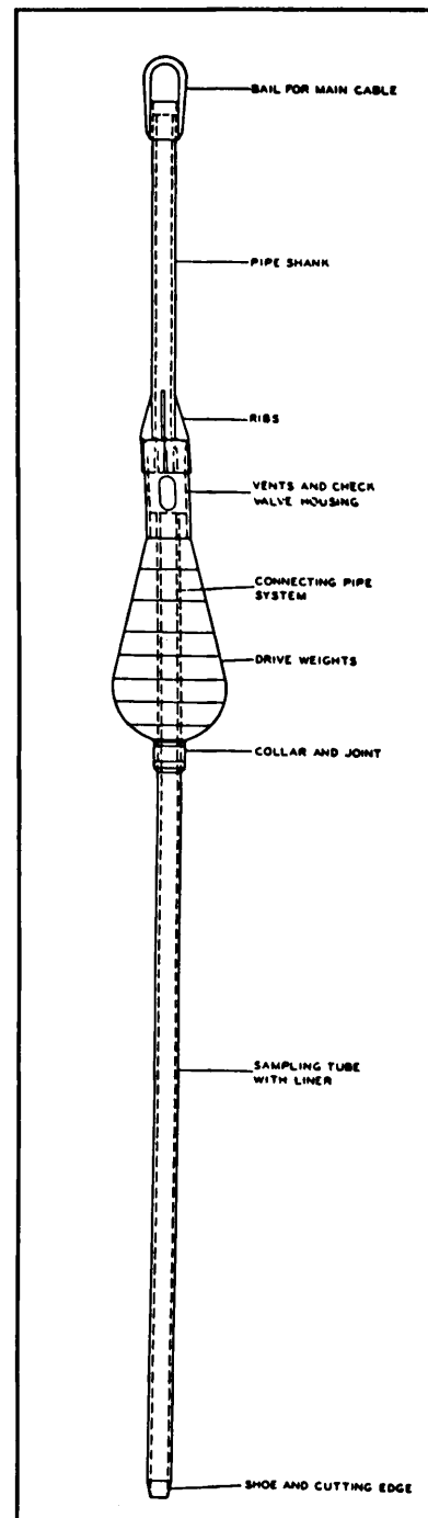
Figure 17. Gravity projectile sampler
