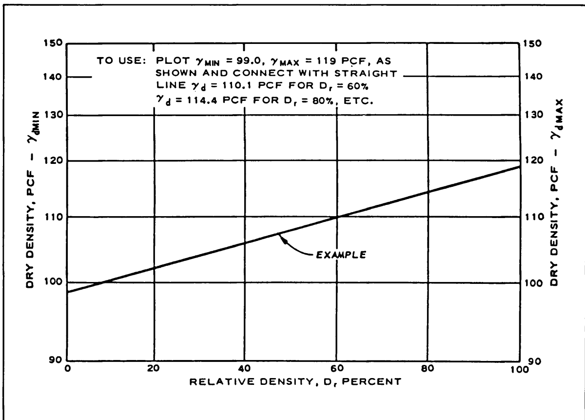
Figure 3. Example of graphical solution for relative density
