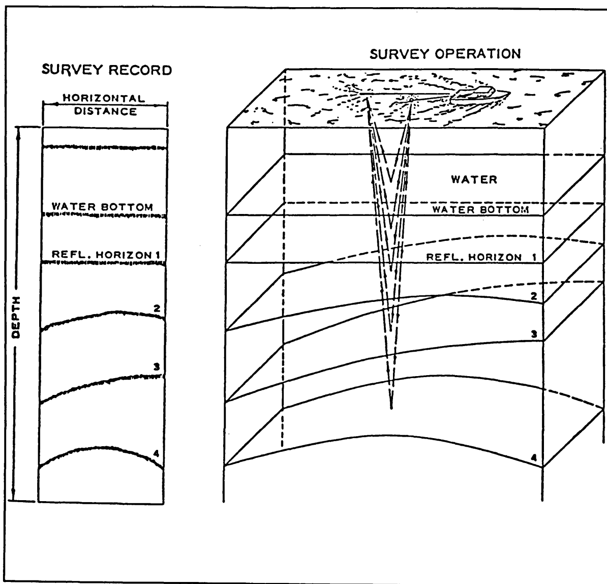
Figure 14. Geophysical acoustic sounding.
