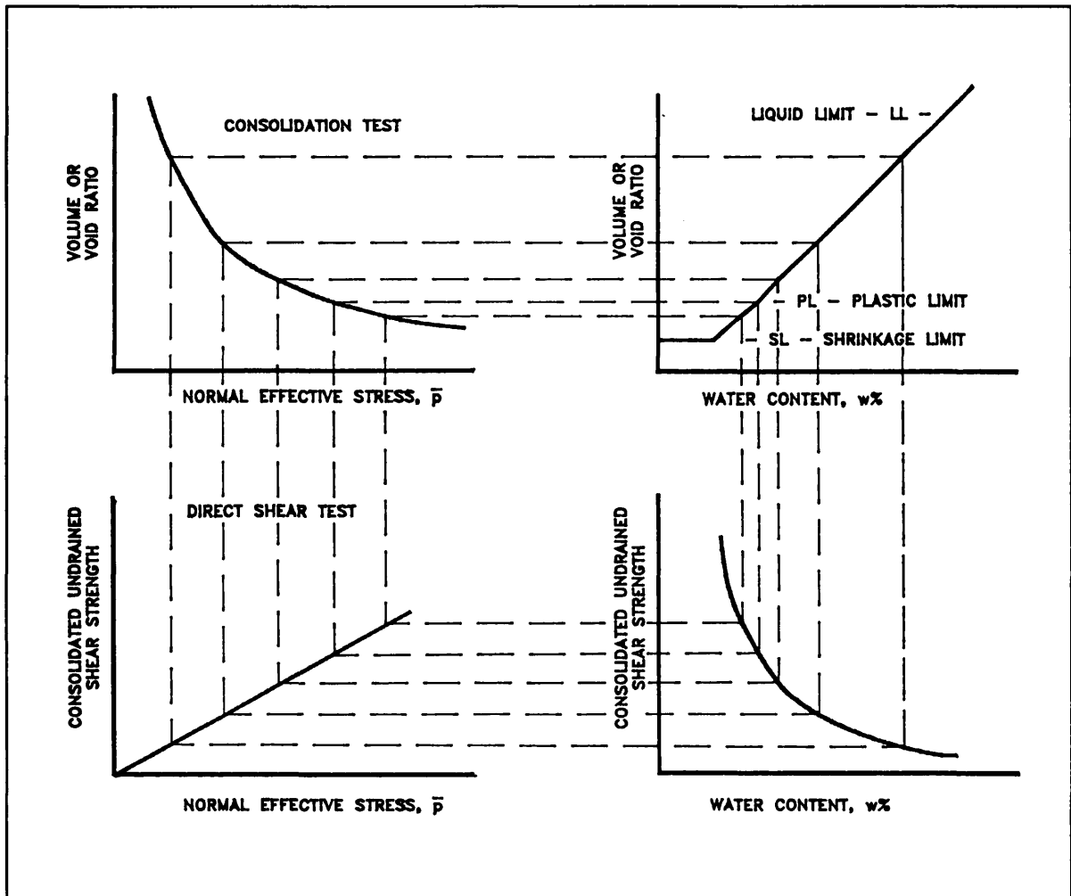
Figure 10. Interrelationship of properties of clay soils
