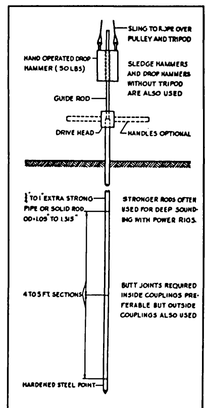
Figure 29. Simple light sounding rod (After Hvorslev 1949)
