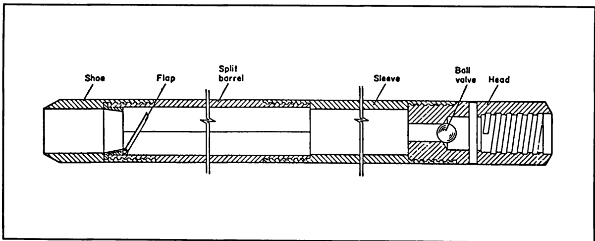
Figure 16. Split tube sampler used in the Standard Penetration Test.
