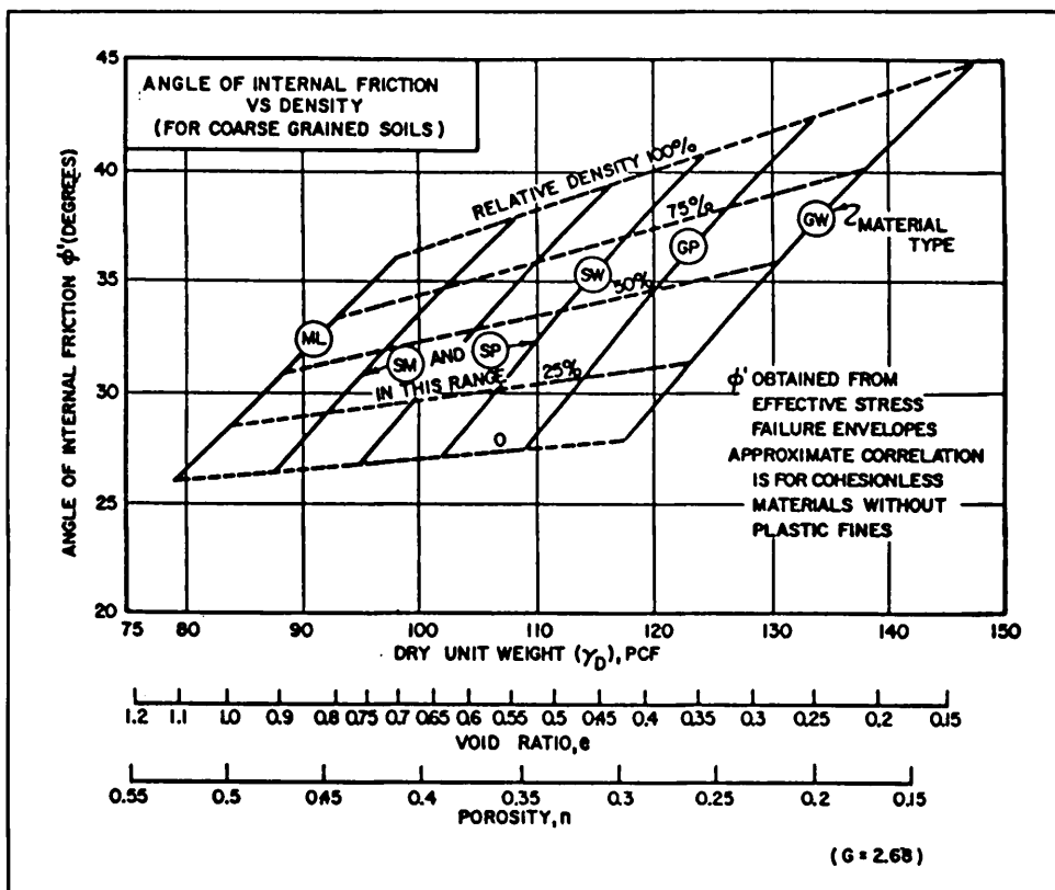
Figure 8. Correlation of strength properties for granular soil
