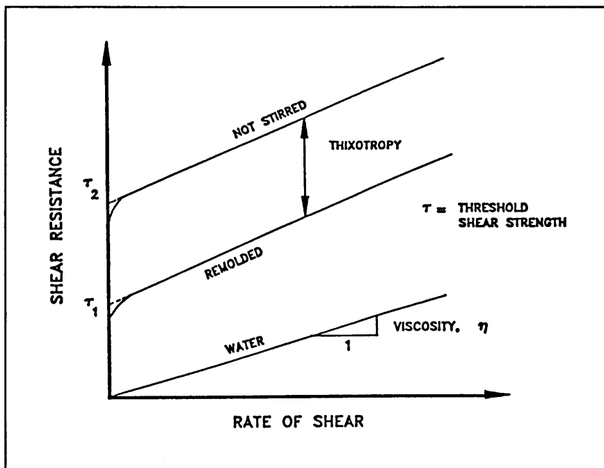
Figure 11. Rheologic behavior of a silt-clay slurry
