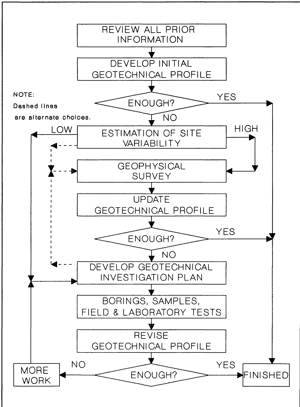
Figure 13. Procedure for a geotechnical site investigation.
