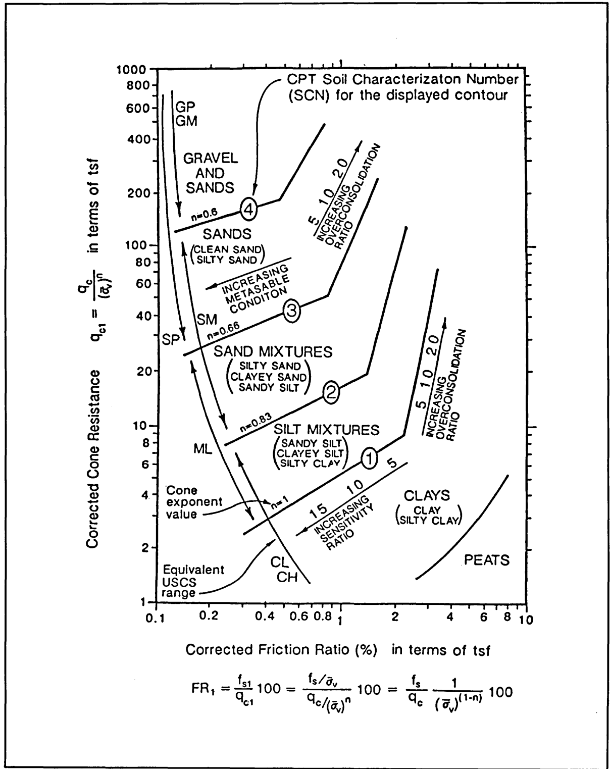
Figure 26. Estimation of soil description from CPT data (After Olsen and Malone 1988)
