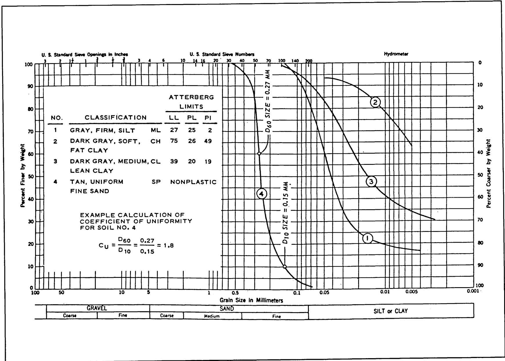
Figure 1. Typical grain-size distribution curves
