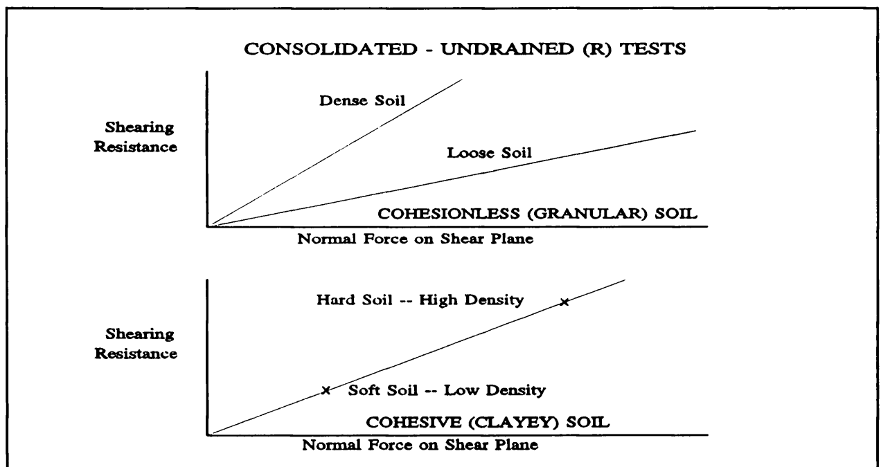
Figure 6. Relationship of shear strength and normal force
