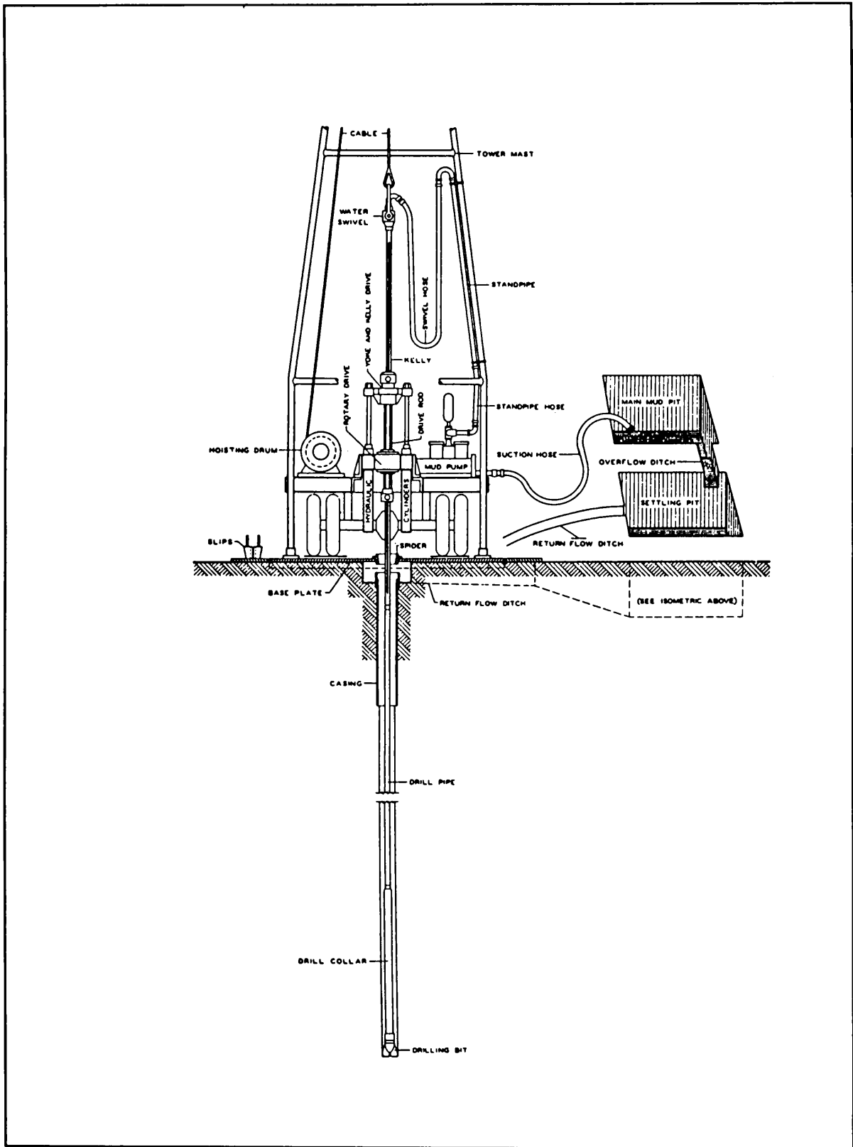
Figure 20. Rotary drilling system
