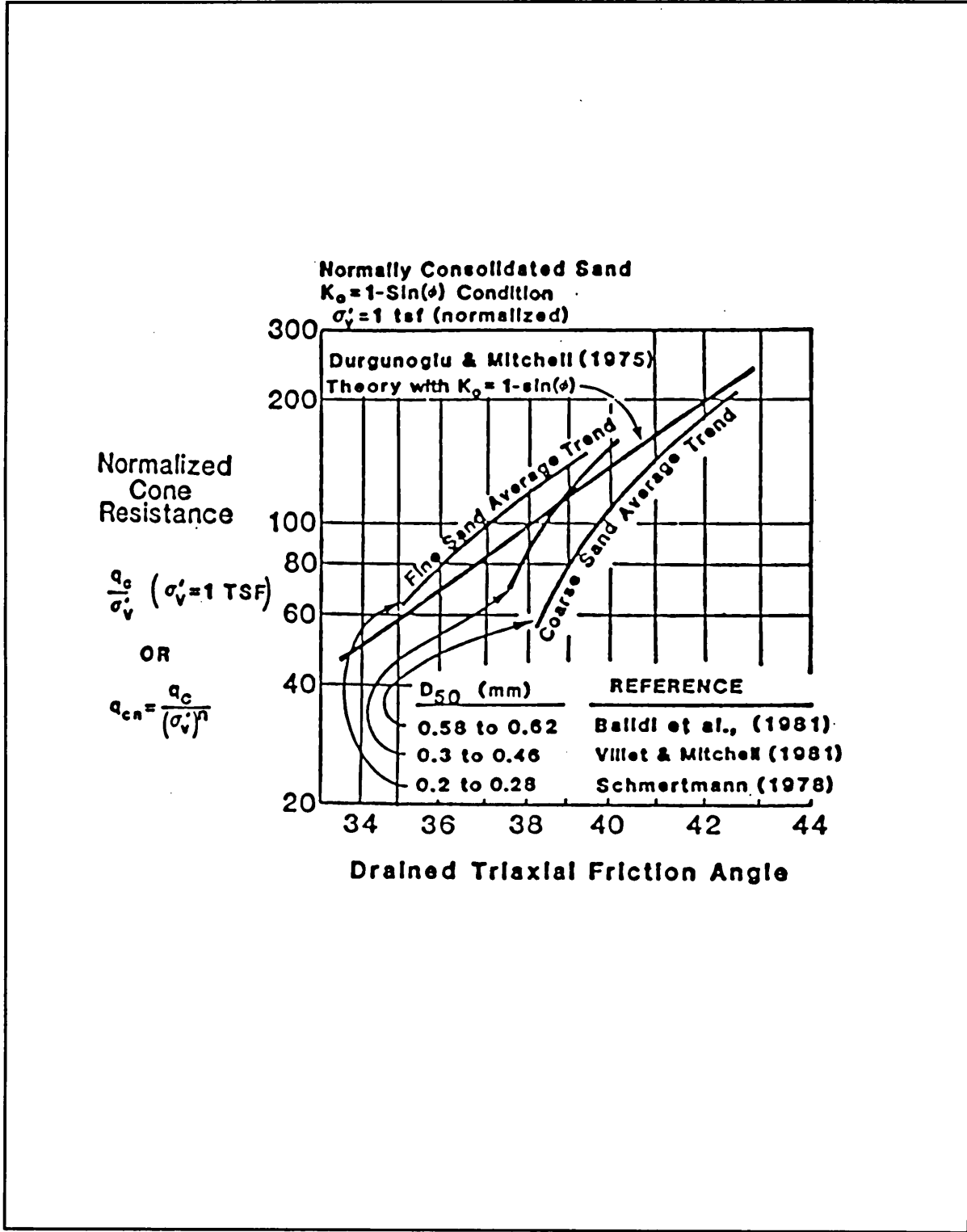
Figure 27. Estimation of angle of friction using CPT data (After Olsen and Farr 1986)
