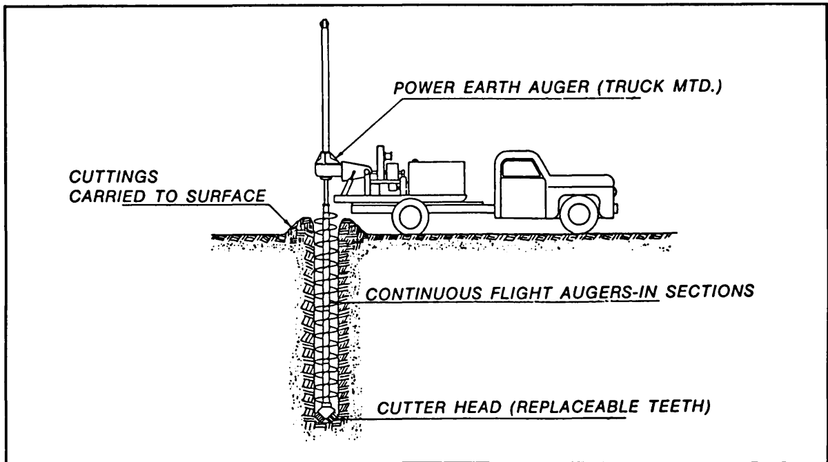
Figure 21. Continuous flight auger drilling system
