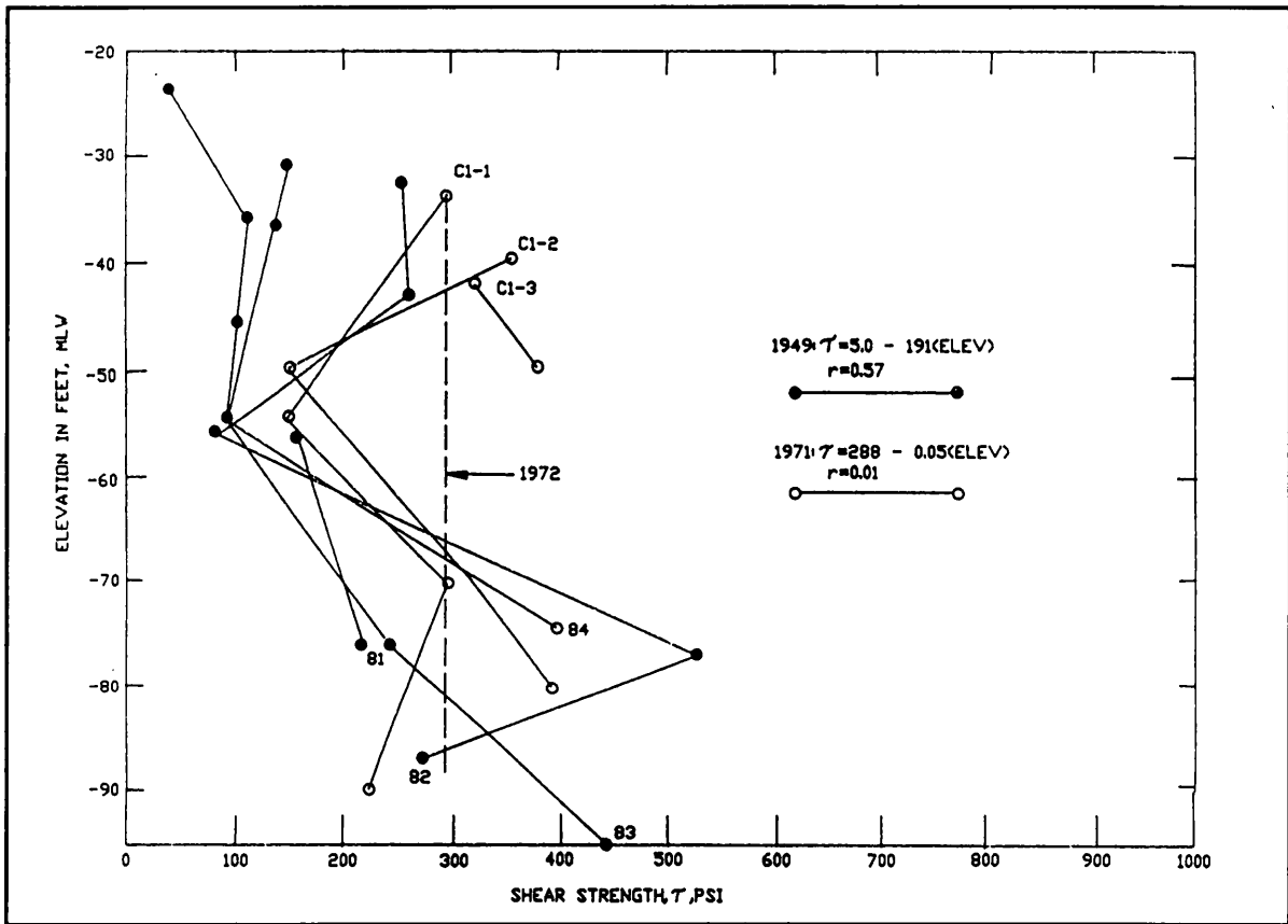
Figure 32. Variation in strength with depth in a marine clay
