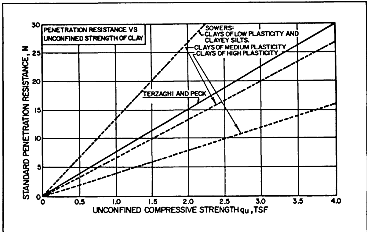
Figure 24. Unconfined compressive strength estimated from SPT N-values
