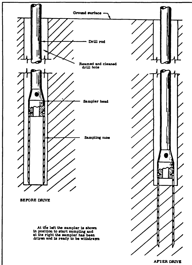
Figure 15. Schematic of thin wall tube sampler
