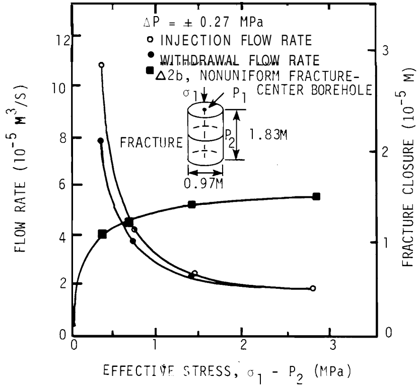
FIGURE 43. Flow Rate and Fracture Aperture Closure as a Function of Effective Stress for a Horizontal Saw-Cut Fracture in a Granite Cylinder (Port-Keller and Gnirk 1981)
