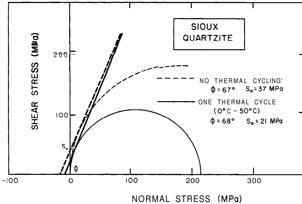
FIGURE 17. Mohr Failure Envelopes for Sioux Quartzite (Fossum 1982)
