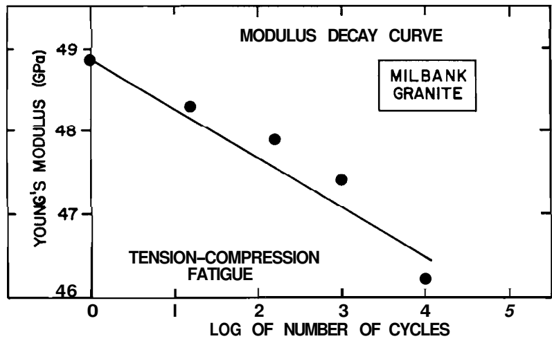
FIGURE 19. Modulus Decay Curve for Milbank Granite (Fossum 1982)
