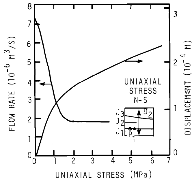
FIGURE 43. Flow Rate and Fracture Aperture Closure as a Function of Effective Stress for a Horizontal Saw-Cut Fracture in a Granite Cylinder (Port-Keller and Gnirk 1981)
