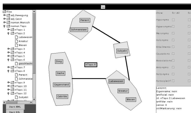
Fig. 10: User Interface to the wordnet visualization tool
