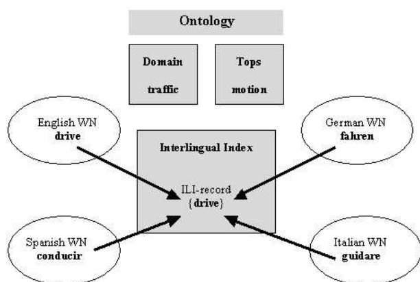
Fig 6: Partial architecture of the EuroWordNet database
