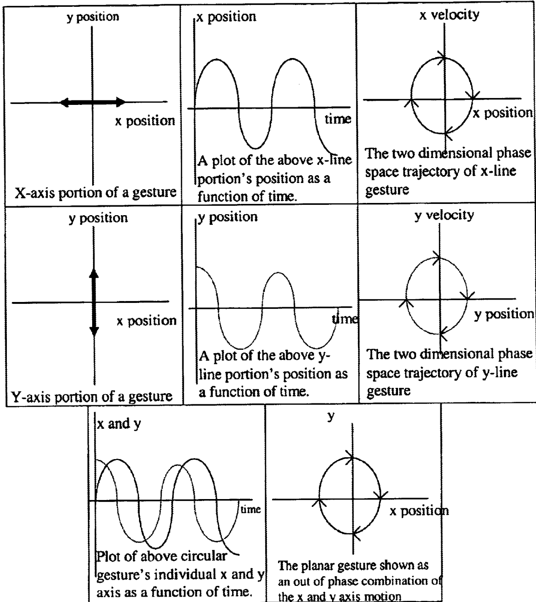
Figure 22: Two Perpendicular Oscillatory Line Motions Combined into a Circular Gesture.
