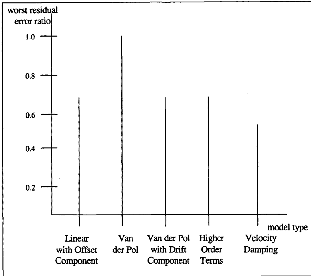
Figure 21: The Worst Case Residual Ratios for Each Gesture Model. The Lower the Ratio, the Better the Model.
