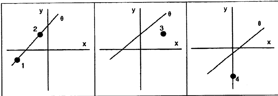
Figure 18: The Recursive Linear Least Squares Method for Updating q with Each Additional (x_i, y_i) Data Point.
