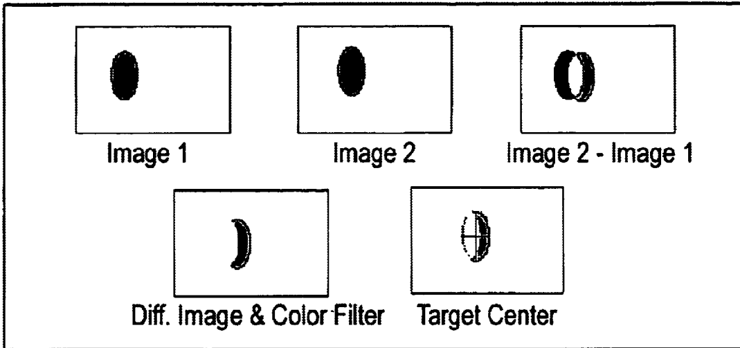
Figure 29: Target Center from Difference Image.
