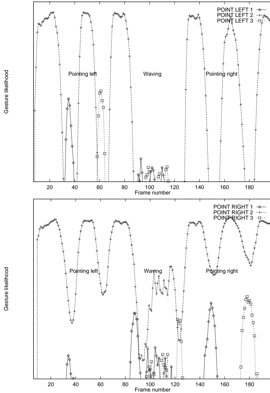
Figure 7: Event likelihoods estimated from the test sequence in Figure 6. The vertical axis is a logarithmic scale. Top: Likelihoods for the pointing left events. Bottom: Likelihoods for the pointing right events.
