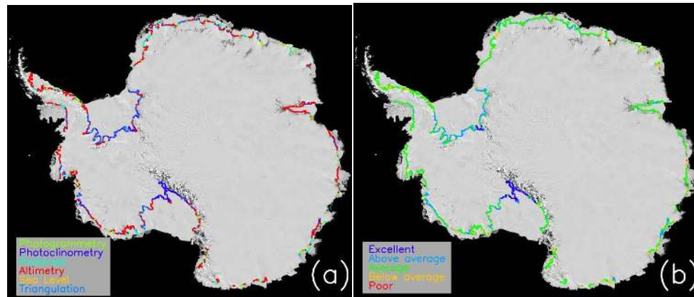
Fig. 7. The AS AID hydrostatic line. (a) Colored lines represent the DEM source of selected elevation values. The corresponding percent frequencies of occurrence are: photogrammetry (green, 4 %); photoclinometry (dark blue, 37 %); Radarsat (cyan, 16 %); altimetry (red, 38 %); sea level (orange, 0.3 %); and triangulation (light blue, 5 %). (b) Colored lines represent the confidence in the selected elevations. The corresponding percent frequencies of occurrence are: Excellent (dark blue, 4 %); Above Average (cyan, 32 %); Average (green, 59 %); Below Average (orange, 4 %); and Poor (red, 0.1 %).
