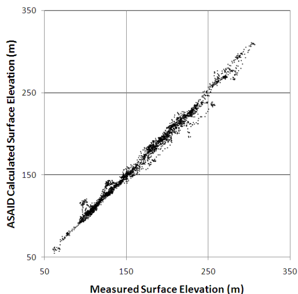
Fig. 8. Surface elevations measured by British Antarctic Survey near grounded ice boundary of Ronne Ice Shelf versus surface elevations at the same locations extracted from a photoclinometry DEM produced by ASAIID.
