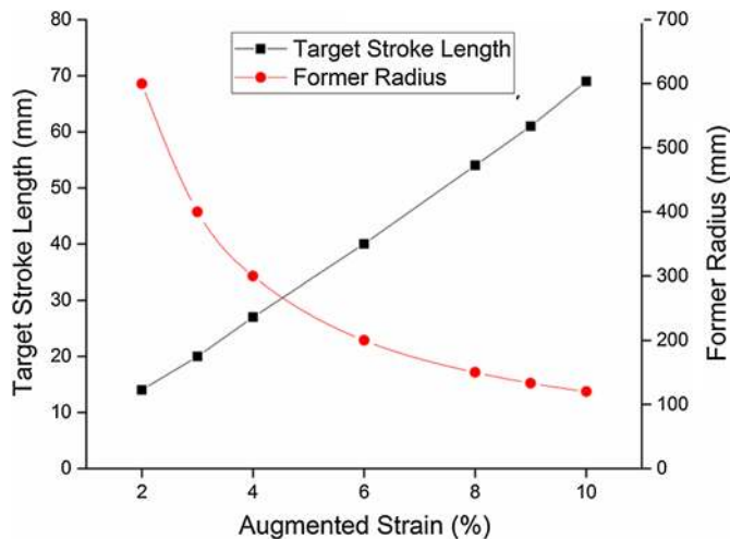
Fig. 23—Comparison of stroke lengths for each experiment.
