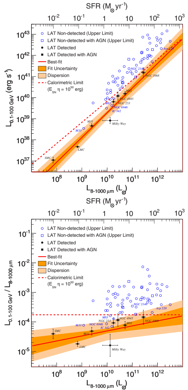
Figure 4. Same as Figure 3, but showing gamma-ray luminosity (0.1–100 GeV) vs. total IR luminosity (8–1000 μm). IR luminosity uncertainties for the non-detected galaxies are omitted for clarity, but are typically ~0.06 dex. The upper abscissa indicates SFR estimated from the IR luminosity according to Equation (1) (Kennicutt 1998b).
