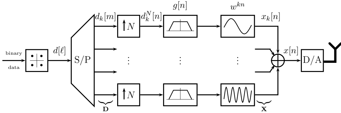
Fig. 1. GFDM transmitter system model
