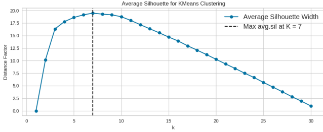
(a) MovieLens 100K - Average Silhouette on K-Mean
