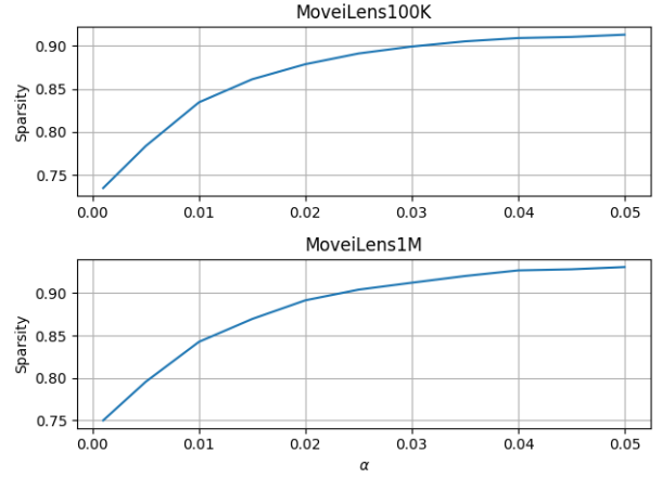
Figure 6: Sparsity of combined features' dataset vs. \alpha before dimension reduction
