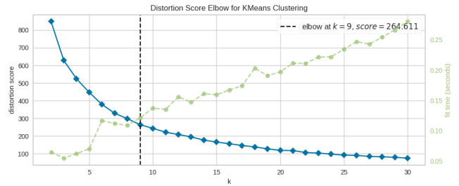
(b) MovieLens 1M - Elbow Method on K-Mean
