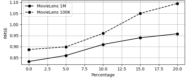
Figure 13: GHR method RMSE result versus the percentage of users which have been randomly removed from the user-item rating matrix.
