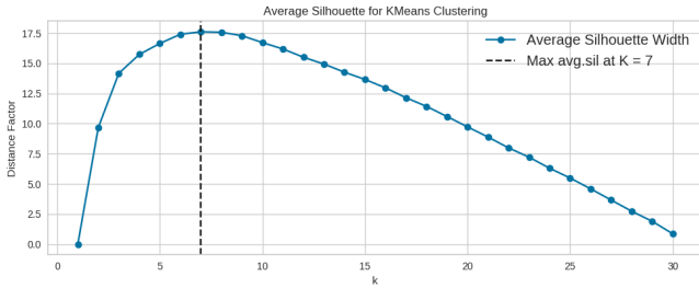
(b) MovieLens 1M - Average Silhouette on K-Mean
