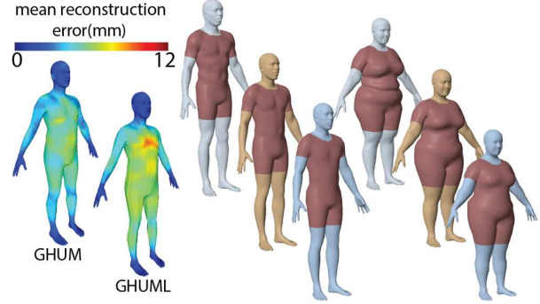
Figure 4. Evaluation on Caesar. Left: Per-vertex Euclidean error to the registration for GHUM and GHUML. Right: (top to bottom, registrations, GHUM and GHUML) VAE-based models can represent body shape very well. Compared to GHUML additional, e.g. muscle or waist, soft tissue detail is preserved by GHUM.
