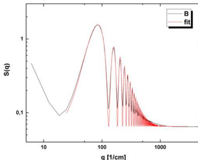
Fig. 6 Static power spectrum of a sequence of shadowgraph images collected during thermodiffusion in binary mixture for \Delta T = 20 K. The red line is the best fit by using available theoretical models
