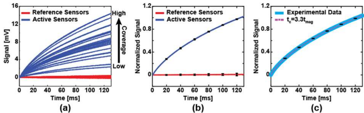
Figure 3. (a) Measured MRX signals from active sensors (blue, n = 29 ) and reference sensors (red, n = 20 ). The different amplitudes indicate non-uniform MNP coverage. (b) Normalized relaxation signals demonstrating the homogeneous relaxation behavior. The curves are the mean signal of reference sensors and active sensors, respectively. Error bars are \pm 1\sigma . (c) Comparison between experimental data and simulation exhibits good consistency of the characteristic time of 3.3t_{mag} . Error bars are \pm 1\sigma .
