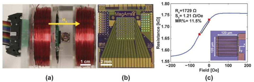
Figure 2. (a) Simplified measurement setup with electromagnet and sensor array. (b) Photograph of GMR sensor array. (c) Optical microscope image of a GMR sensor and measured magnetoresistance curve.
