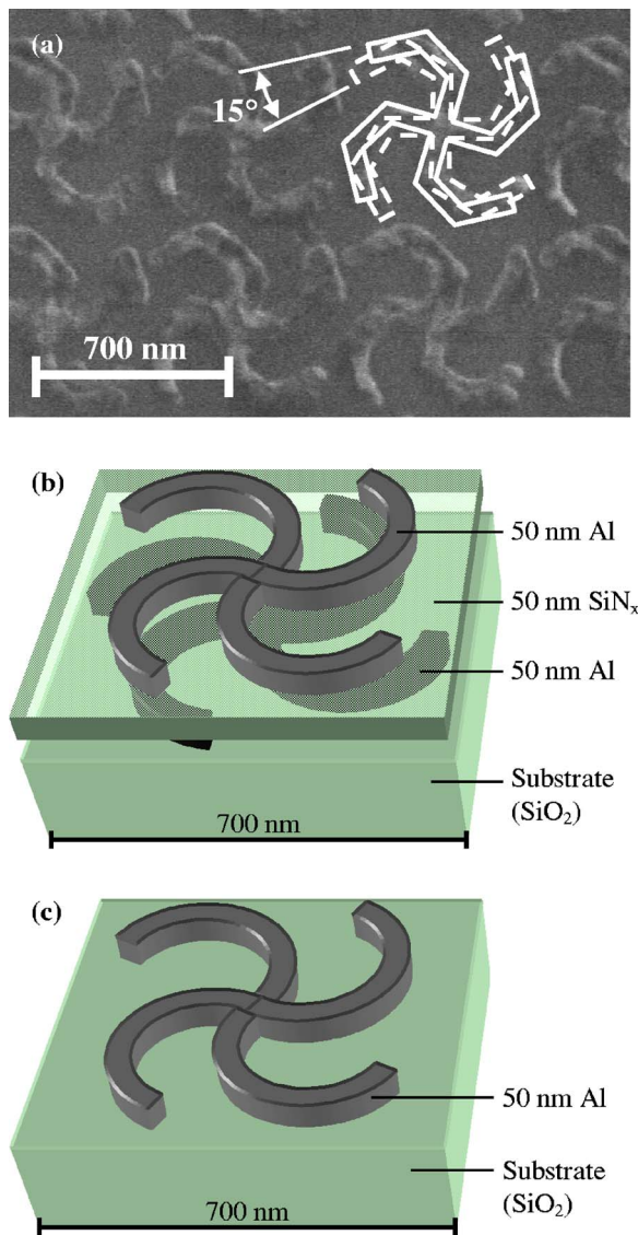
FIG. 1. (Color online) (a) SEM micrograph of the bilayered metamaterial. Note that the rosettes in two layers are mutually twisted and that their centers are aligned with high precision. (b) Schematics of the bilayered metamaterial's square unit cell. (c) Schematics of the monolayered reference metamaterial's square unit cell.
