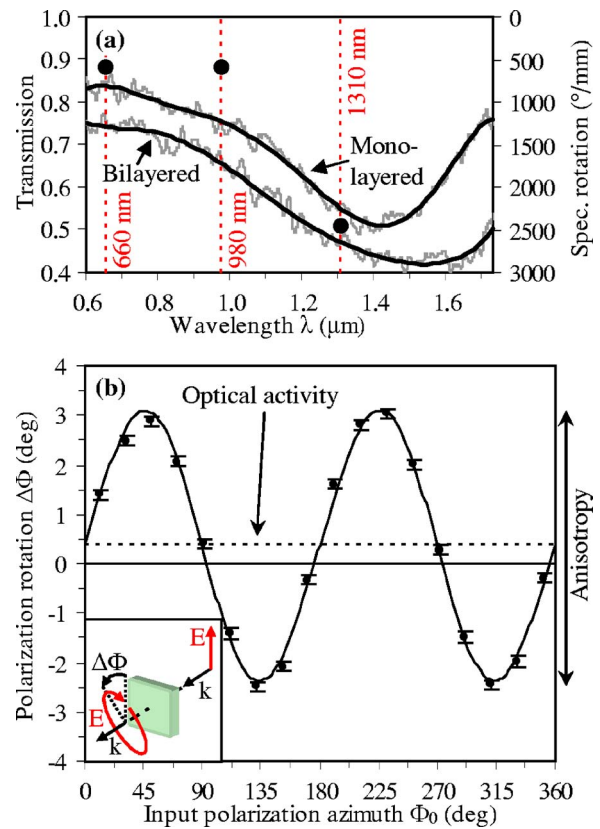
FIG. 2. (Color online) (a) Transmission spectra of the bilayered and reference monolayered metamaterial structures. Red dashed lines indicate wavelengths for which the optical activity has been measured and black dots mark the specific rotation of the bilayered metamaterial at these wavelengths. (b) Polarization rotation induced by the bilayered metamaterial at 1310 nm as a function of azimuth of the incident linearly polarized light. The solid line is a numerical fit. The dashed line indicates the true level of the optical activity component in the rotation.
