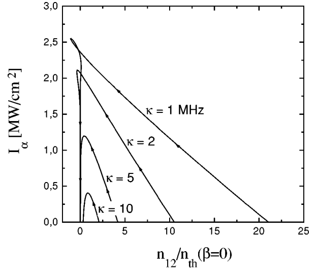
FIG. 5. Intensity of the generated laser pulses along time evolution as a function of the relative amount of population difference above the threshold population inversion for different values of the cavity losses \kappa .
