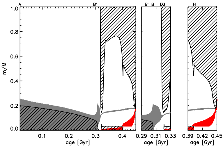
Fig. 5 Kippenhahn diagram of a 3 M_{\odot} model as shown in Fig. 3. Regions where convection takes place are hatched. Regions where nuclear burning produces more than 10 \text{ erg g}^{-1} \text{ s}^{-1} are shown in grey for hydrogen burning and in red in case of helium burning. The central panel shows a zoom of the subgiant and red-giant branch. The right panel shows a zoom of the late stages of evolution. The letters at the top indicate different stages of evolution corresponding to the phases indicated in Fig. 3
