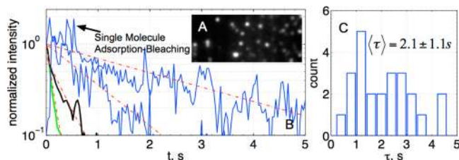
Figure 2. (a) One frame from a video measuring the lifespan of fluorescent molecules. The bright spots are fluorescence from the molecules on the nanoantennas. (b) The blue curves are decays of fluorescence from two bright spots due to the photobleaching. The red dash-dot lines are fit to a single exponential decay, yielding the decay constants of 0.97 \pm 0.09 s and 2.76 \pm 0.07 s, respectively. The power of the excitation laser is 10 mW. As a comparison, we plot the fluorescence decay of the same molecules on a quartz surface at a 10 mW (black) and 40 mW (green) excitation intensity respectively, in the same figure. The bleaching on the antennas is much slower. (c) A histogram of the fitted decay constants from 24 antennas, yields an averaged lifespan of 2.1 s, which is a 5-fold improvement comparing to the same molecules at the same excitation intensity ( \sim 0.4 s shown in Figure 1b).
