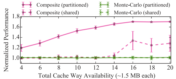
(b) Composite-Scimark (cache-utilizer) performance drops when sharing cache with Monte-Carlo (cache-neutral, does not gain from extra cache). Therefore, we consider Monte-Carlo to be a cache-polluter.
