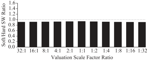
(a) Both applications are H.264 . Hard-partitioning yields better social welfare than soft-partitioning for all ratios.
