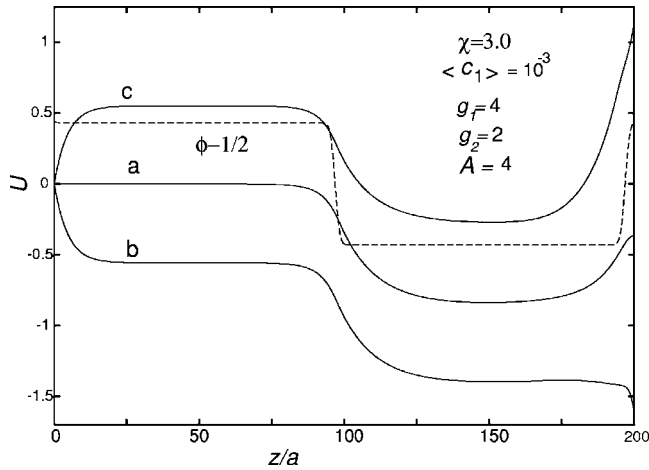
FIG. 2. Normalized electric potential U(z)=e\Phi(z)/k_B T between parallel plates with L=200a , where we set \Phi(0)=0 . The surface charge \sigma_0(=-\sigma_L) is 0 (a), 2.5 \times 10^{-3} e/a^2 (b), and -2.5 \times 10^{-3} e/a^2 (c). The curve of \psi(z)=\phi(z)-1/2 (broken line) indicates the presence of an interface in the middle and a wetting layer in contact with the wall at z=L .
