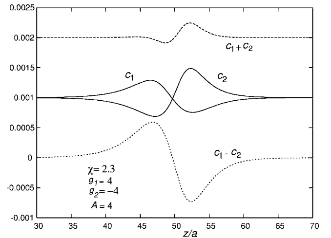
FIG. 15. Normalized ion densities c_1 and c_2 around an interface, where g_1=4 , g_2=-4 , \chi=2.3 , and A=4 . The first species is hydrophilic and the second one is hydrophobic. Also shown are c_1 - c_2 = a^3 \rho / e and c_1 + c_2 = a^3 n . A marked electric double layer is formed here.
