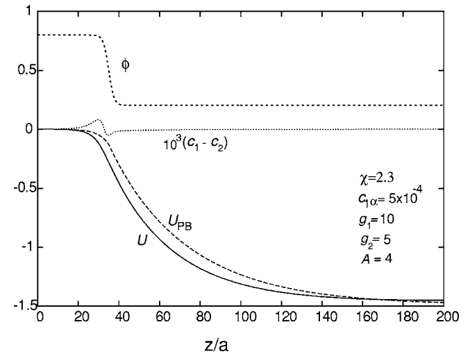
FIG. 13. Normalized electric potential U(z) = e\Phi(z)/k_B T (solid line) at small ion density c_{1\alpha} = 5 \times 10^{-4} with \chi = 2.3 , g_1 = 10 , g_2 = 5 , and A = 4 . Here c_{1\beta} = 5.9 \times 10^{-6} and \kappa_\beta = 2.5 \times 10^{-2} . It is compared with the Poisson-Boltzmann solution, Eqs. (4.55) and (4.56), without the image interaction. Also shown are composition profile \phi(z) and the scaled charge density 10^3[c_1(z) - c_2(z)] .
