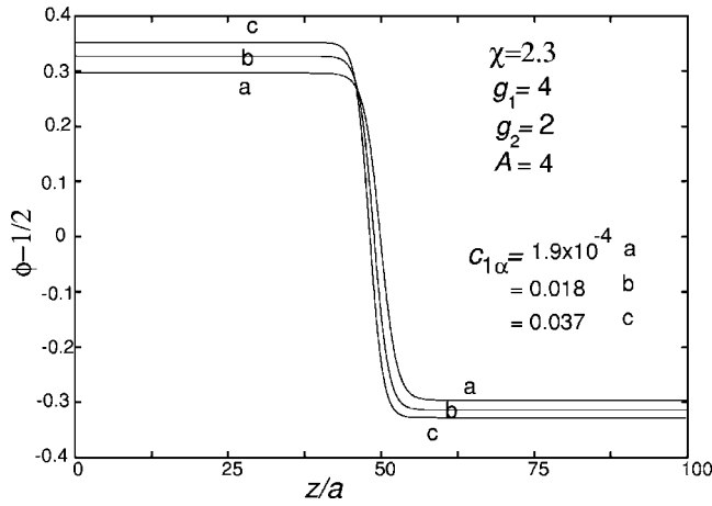
FIG. 5. Order parameter profile \psi(z) = \phi(z) - 1/2 for three cases of c_{1\alpha} = 1.9 \times 10^{-4} (a), 0.018 (b), and 0.037 (c). For the smallest c_{1\alpha} , \psi(z) is almost equal to the profile without ions.
