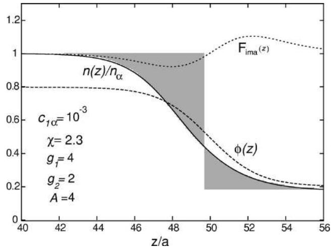
FIG. 8. Normalized ion density n(z)/n_\alpha , composition \phi(z) , and image factor F_{\text{ima}}(z) for \chi=2.3 , g_1=4 , g_2=2 , and c_{1\alpha}=10^{-3} . The gray regions correspond to the two terms in Eq. (4.45).
