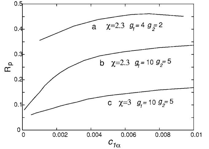
FIG. 14. Potential reduction ratio in the \alpha region R_p = [\Phi_\alpha - \Phi(z_{\text{int}})] / (\Phi_\alpha - \Phi_\beta) versus c_{1\alpha} , where \chi=2.3 , g_1=4 , and g_2=2 (a), \chi=2.3 , g_1=10 , and g_2=5 (b), and \chi=3 , g_1=10 , and g_2=5 (c).
