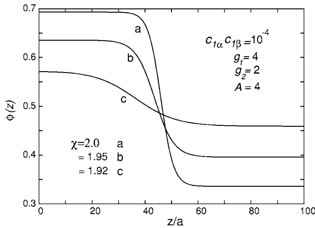
FIG. 11. Composition profiles with varying \chi for g_1=4 , g_2=2 , A=4 , and v_0\bar{n}=0.02 , for which \chi_c^{\text{ion}}=1.91 .
