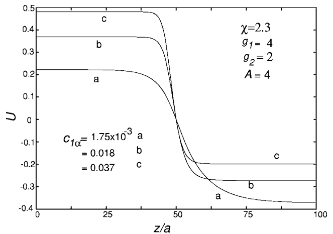
FIG. 4. Normalized electric potential U(z) = e\Phi(z)/k_B T for three cases of c_{1\alpha} = 1.75 \times 10^{-3} , 0.018, and 0.037, where we set \Phi(50a) = 0 .
