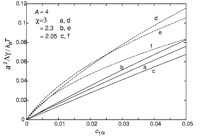
FIG. 6. Normalized excess surface tension a^2\Delta\gamma/k_B T vs c_{1\alpha} for \chi=3 (a), 2.3 (b), and 2.05 (c) with g_1=4 and g_2=2 (solid lines), and for \chi=3 (d), 2.3 (e), and 2.05 (f) with g_1=10 and g_2=5 (broken lines).
