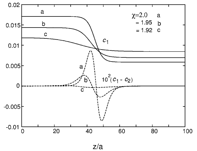
FIG. 12. Normalized ion density c_1(z) and normalized charge density c_1(z) - c_2(z) (multiplied by 100) with varying \chi with the same parameter values as in Fig. 11.
