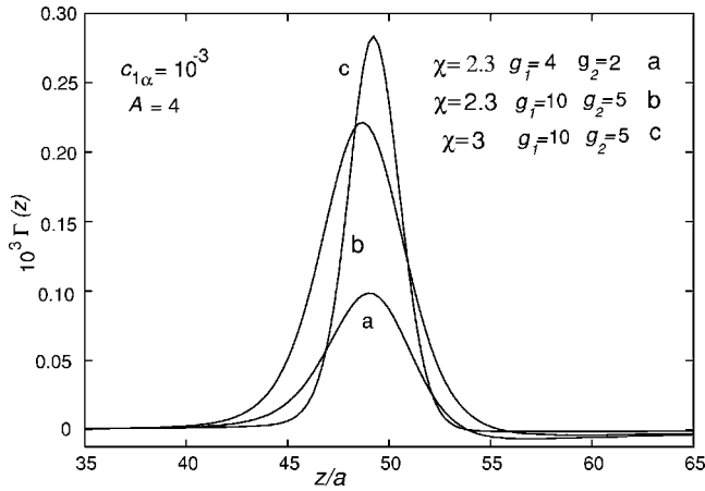
FIG. 7. Normalized integrand \Gamma(z) of Eq. (4.41) for \chi=2.3 , g_1=4 , and g_2=2 (a), for \chi=2.3 , g_1=10 , and g_2=5 (b), and for \chi=3 , g_1=10 , and g_2=5 (c). Its integral with respect to z/a is equal to a^2 \Delta \gamma / k_B T in the approximate formula (4.40).
