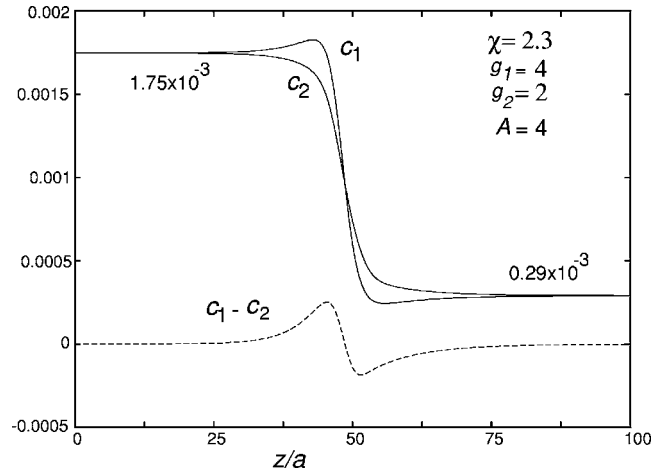
FIG. 3. Normalized ion densities c_1(z) and c_2(z) around an interface where c_{1\alpha} = c_{2\alpha} = 1.75 \times 10^{-3} and c_{1\beta} = c_{2\beta} = 0.29 \times 10^{-3} .
