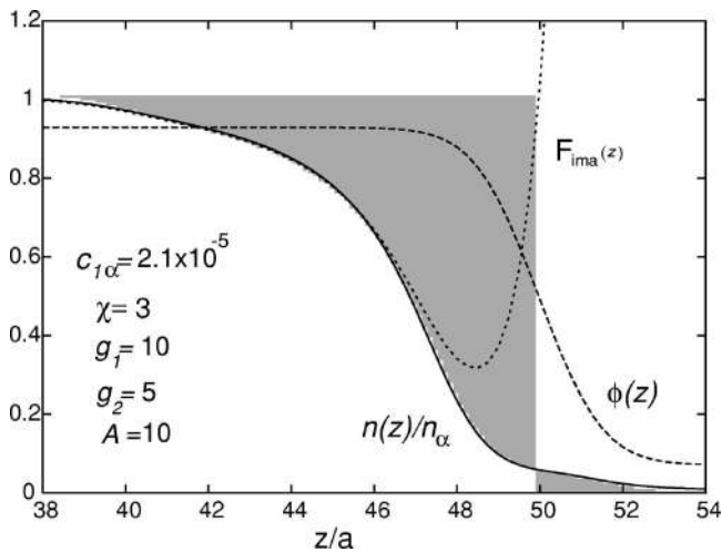
FIG. 10. Normalized ion density n(z)/n_\alpha , composition \phi(z) , and image factor F_{\text{ima}}(z) for \chi=3 , g_1=10 , g_2=5 , and c_{1\alpha}=2.1 \times 10^{-5} . For these parameters, the role of the image factor on n(z) is more dominant than that of the solvation interaction.
