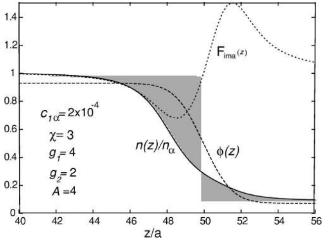
FIG. 9. Normalized ion density n(z)/n_\alpha , composition \phi(z) , and image factor F_{\text{ima}}(z) for \chi=3 , g_1=4 , g_2=2 , and c_{1\alpha}=2 \times 10^{-4} .
