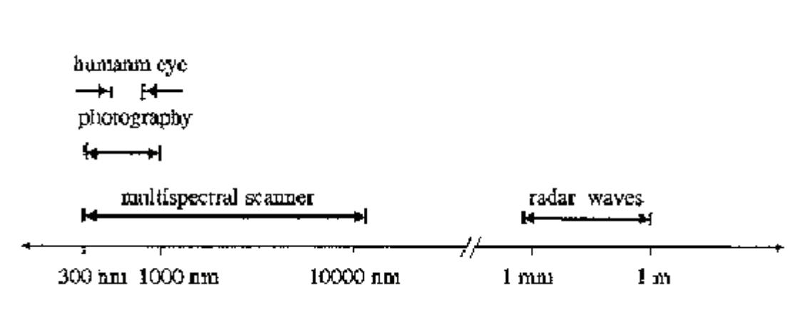
Figure 4. The electromagnetic spectrum
