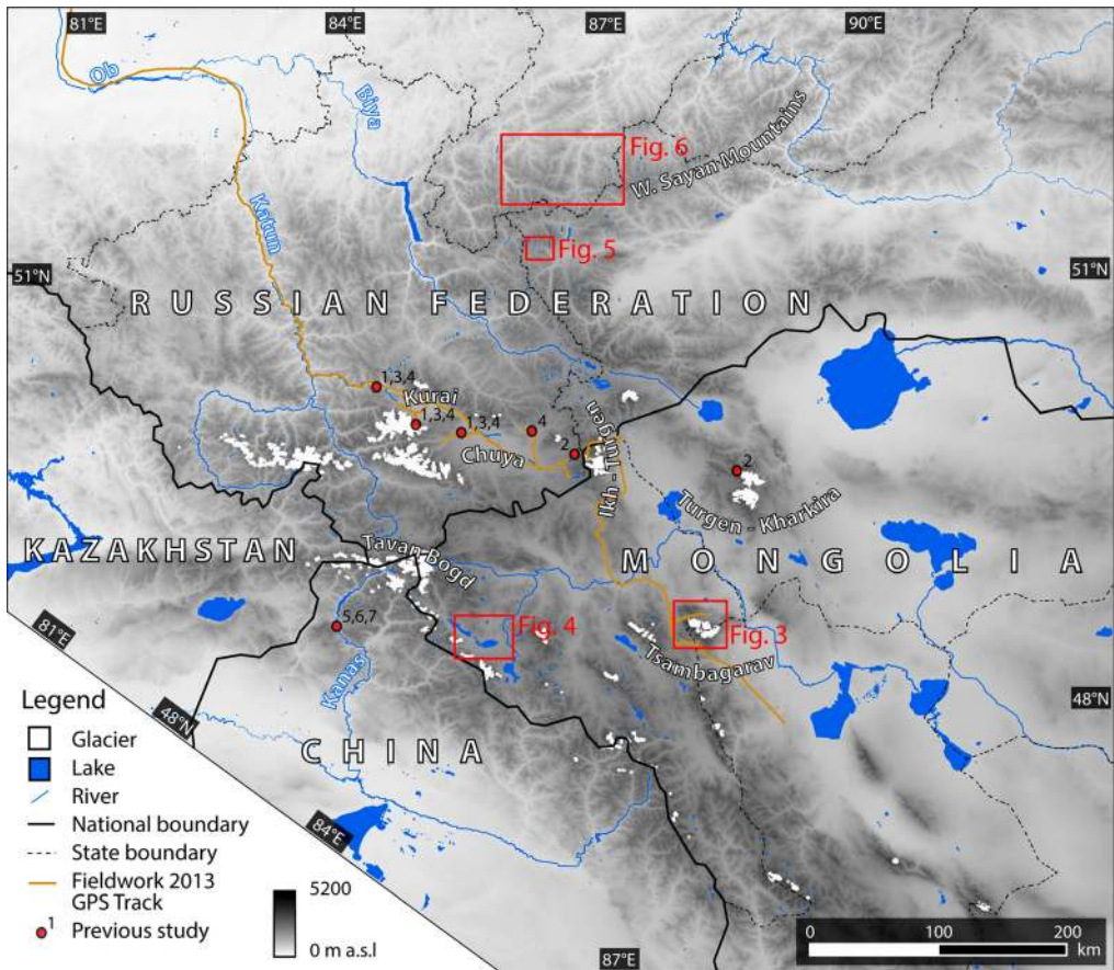
Figure 2. Physiography and administrative borders of the Altai region. The locations of previous studies of paleoglaciation and glacial geomorphology are shown: (1) Rudoy (2002), (2) Lehmkuhl et al. (2004), (3) Herget (2005), (4) Reuther et al. (2006), (5) Xu et al. (2009), (6) Xu et al. (2010), and (7) Zhao et al. (2013). Red boxes with numbers denote the locations of Figures 3–6. The background topographic data consist of the Aster Global Digital Elevation Model (AGDEM). Contemporary glacier extent is from the Randolph Glacier Index (RGI) (Arendt et al., 2012).
