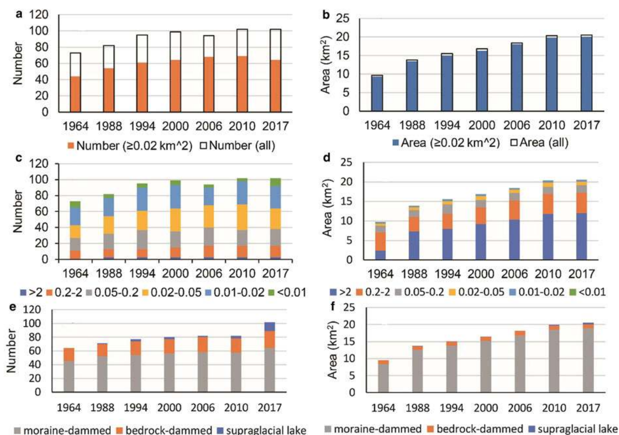
Fig. 2. Number and area changes from 1964 to 2017 for lakes identified visually from Landsat imagery. (a) Number change for all lakes and lakes with area \geq 0.02 \text{ km}^2 . (b) Area change for all lakes and lakes with area \geq 0.02 \text{ km}^2 . (c) Number change for lakes in different size divisions. (d) Area change for lakes in different size divisions. (e) Number change for lake classification (moraine-dammed, bedrock-dammed and supraglacial lake). (f) Area change for lake classification (moraine-dammed, bedrock-dammed and supraglacial lake).
