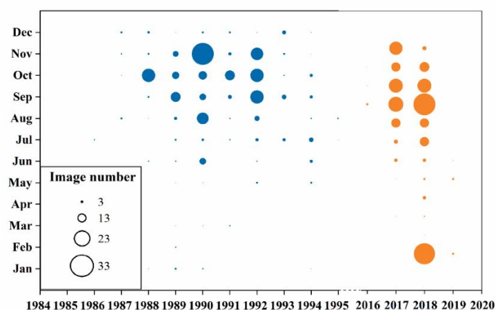
Figure 2. Time phases of remote sensing images selected for High Mountain Asian glacial lake inventory.
