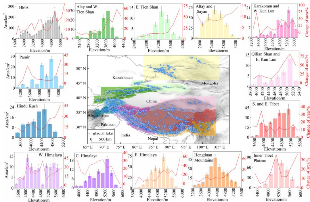
1 2 Figure 7. Distribution and change of glacial lake area in the entire HMA and its 13 sub-regions from 3 1990–2018. 4
