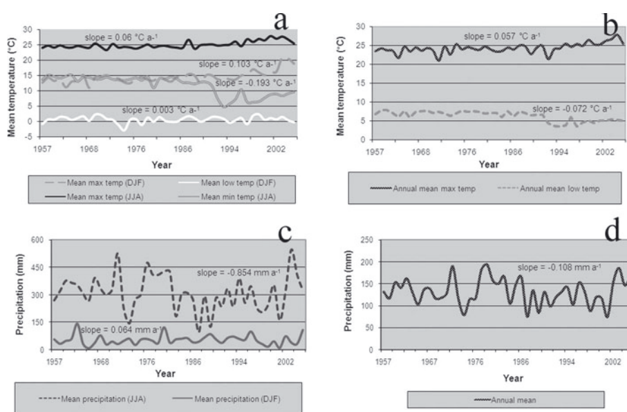
Fig. 8. Climate parameters for Mukhim station: (a) mean T_{MAX} and T_{MIN} for DJF and JJA from 1957 to 2005; (b) mean annual T_{MAX} and T_{MIN} ; (c) mean minimum and maximum precipitation for DJF and JJA; and (d) annual mean precipitation. DJF: December, January, February; JJA: June, July, August.
