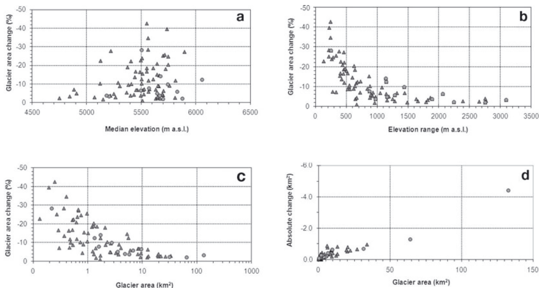
Fig. 7. Scatter plots of (a) median elevation vs glacier area change (%), (b) elevation range vs glacier area change (%), (c) glacier area (km 2 ) vs glacier area change (%) and (d) glacier area (km 2 ) vs absolute glacier area change (km 2 ). Triangles are for the Saraswati/Alaknanda basin and circles are for the Bhagirathi basin. Glacier area change (%) derived from analysis of Corona (27 September 1968) and ASTER (11 October 2006) images.
