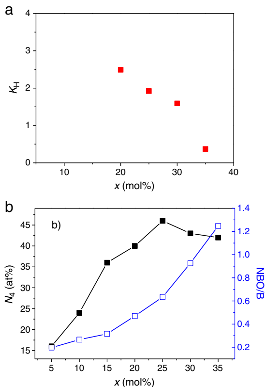
Fig. 11. (a) Hruby parameter ( K_H ) as a function of the \text{Na}_2\text{O} content ( x ) for the four glasses with x=20, 25, 30, and 35 . (b) N_A and \text{NBO/B} as a function of x . The uncertainties in N_A are on the order of \pm 0.2\% and the errors in K_H are around \pm 0.03 .
