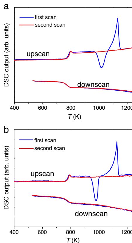
Fig. 8. DSC scans for the glass with x = 20 using (a) 20\text{ K/min} heating and cooling and (b) 10\text{ K/min} heating and cooling.
