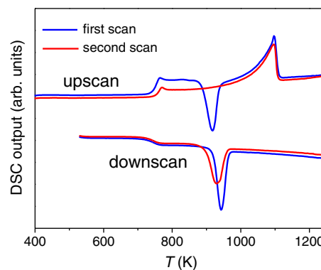
Fig. 9. DSC scans for the glass with x = 30 at 20\text{ K/min} heating and cooling.
