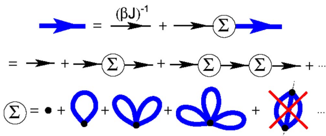
FIG. 1 (color online). For long-range interactions the self-energy \Sigma can be approximated by a local operator. The full propagator is obtained as a simple geometric series. The (thick) lines represent the (renormalized) interaction, the dots one-site correlators.
