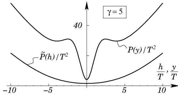
FIG. 2. The distributions \tilde{P}(h) and P(y) of the instantaneous and pseudoequilibrium fields, respectively. Since the latter include the relaxation of the environment, the gap is narrower.
