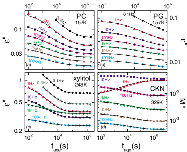
FIG. 3 (color online). (a)–(c) \varepsilon''(t_{\text{age}}) and (d) M''(t_{\text{age}}) of four different glass formers for various frequencies. The lines are fits as described in Fig. 2(a) with \beta_{\text{age}} = 0.6 (PC [11,18]), 0.58 (PG [22,25]), 0.43 (xylitol [22]), and 0.4 (CKN, from structural relaxation [30]).
