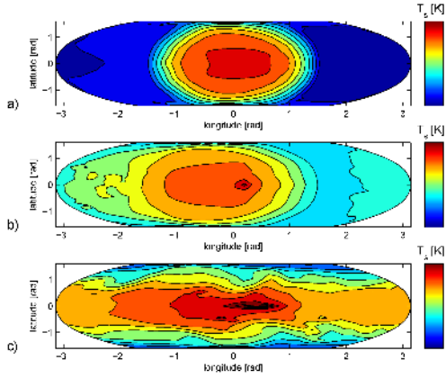
Fig. 1.— Surface temperature snapshots after 60 orbits integration time for rocky planet simulations with a) 1:1, b) 1:2 and c) 1:10 tidal resonance and a 20-bar \text{CO}_2 atmosphere.
