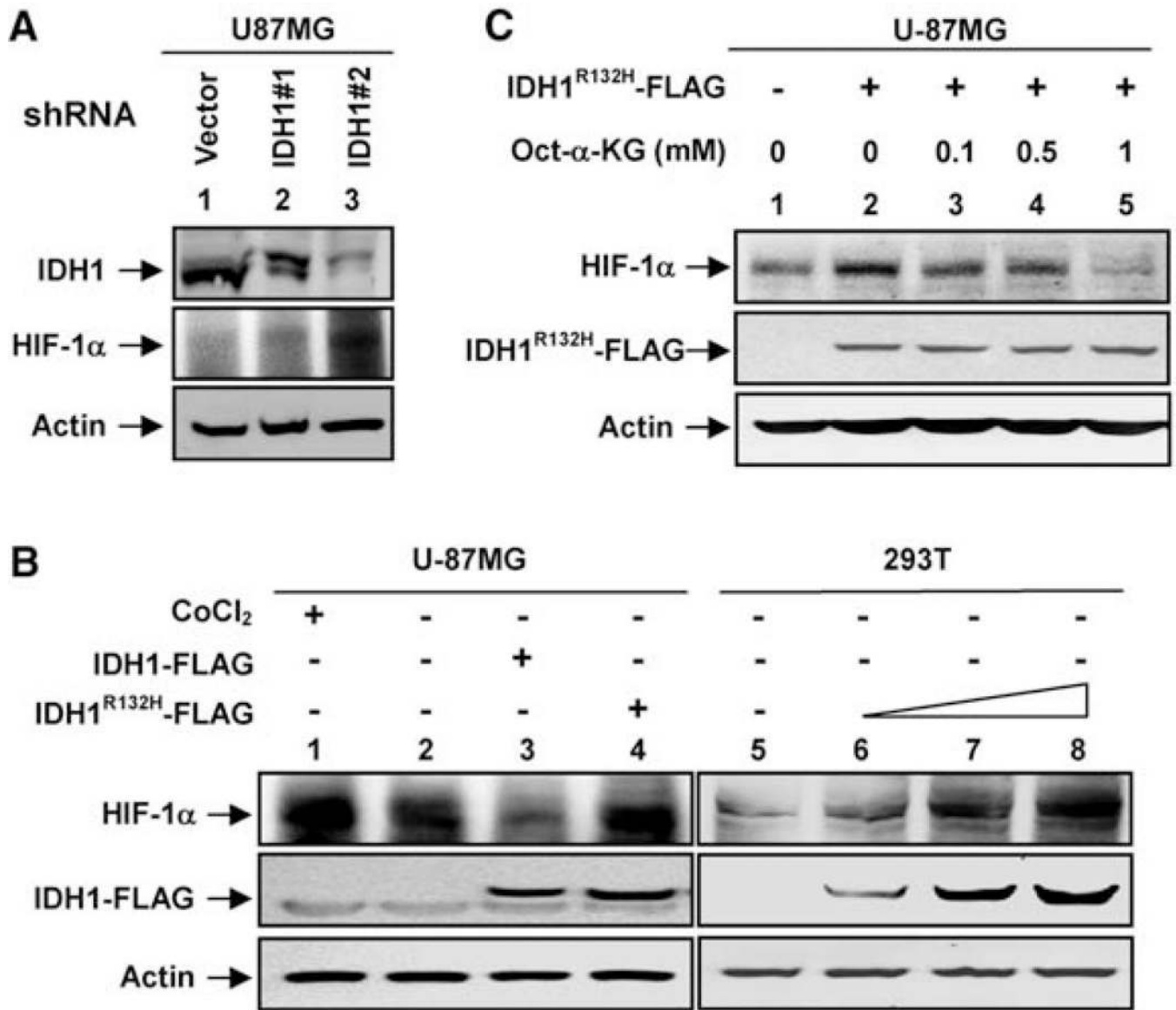
Fig. 3. \alpha -KG mediates the HIF-1 \alpha induction in cells with a decreased IDH1 activity (A) IDH1 knockdown elevates HIF-1 \alpha levels in U-87MG glioblastoma cells. IDH1 and HIF-1 \alpha protein levels were determined by Western blotting from stable U-87MG cells transduced with empty retrovirus or retrovirus expressing different shRNAs silencing IDH1 . (B) Ectopic expression of the IDH1 R132H mutant elevates HIF-1 \alpha levels in U-87MG and HEK293T cells. The IDH1 R132H mutant was overexpressed in U-87MG or HEK293T cells, and protein levels were detected by Western blot. CoCl 2 -treated cells (a mimetic of hypoxia) and cells overexpressing wild-type IDH1 were also included as controls. (C) A cell-permeable \alpha -KG derivative blocks HIF-1 \alpha induction in cells expressing IDH1 R132H . The U-87MG cells were transfected with IDH1 R132H , and different concentrations of octyl- \alpha -KG ester were added to each transfected cell for 4 hours. HIF-1 \alpha protein levels were assayed by Western blot.
