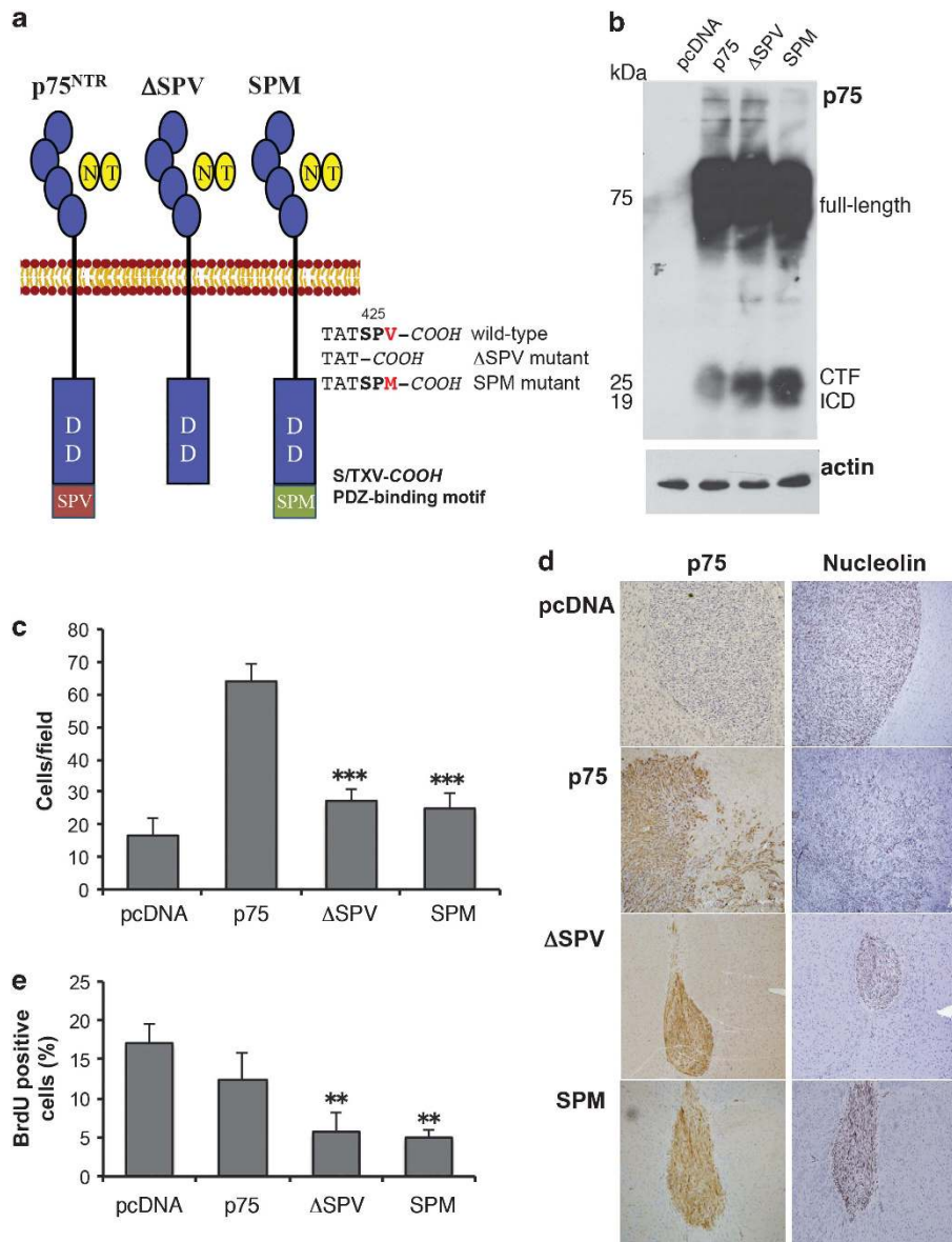
Figure 4. p75 NTR C-terminal PDZ-binding motif is required for glioma invasion in vitro and in vivo . (a) Schematic diagram of the p75 NTR PDZ-binding motif mutants (ΔSPV; SPM). (b) Western blot analysis using a C-terminal domain antibody to p75 NTR confirms the expression of the wild-type (p75) and mutant (ΔSPV; SPM) p75 NTR constructs. Western blot for actin was used as a loading control. (c) Histogram shows the number of U87 p75 NTR wild-type and PDZ-binding mutants (ΔSPV; SPM) that migrated through a collagen-coated transwell. Values are the mean ± s.e.m. from three independent experiments; asterisks (***) indicate P < 0.001 as compared with p75 NTR (one-way ANOVA with the Neuman-Keuls post-test). (d) U87pcDNA, p75 NTR , ΔSPV and SPM glioma cells ( 5 \times 10^4 cells) were implanted intracerebrally into SCID mice and allowed to grow for 28 days. The mice were killed, and paraffin brain sections were stained with human nucleolin and p75 NTR (brown) to visualize the tumors. Sections were counterstained with hematoxylin (blue). (e) Bromodeoxyuridine (BrdU) was injected into the tumor-bearing mice 24 h prior to sacrifice. Frozen brain sections were stained with an antibody against BrdU and counterstained with toluidine blue to visualize the cell nucleus. Histogram represents the percentage of BrdU-positive cells in five consecutive fields. Values shown are the mean ± s.e.m. from five independent mice; asterisks (**) indicate P < 0.01 as compared with U87pcDNA (one-way ANOVA with the Neuman-Keuls post-test).
