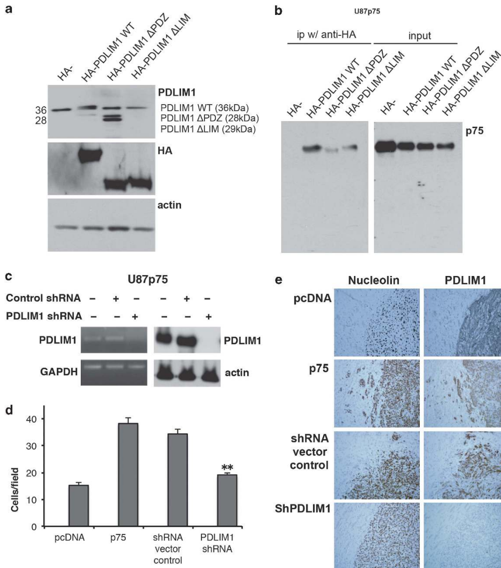
Figure 6. PDLIM1 is critical for glioma cell invasion. (a) U87p75 cells were transfected with full-length HA-PDLIM1 or HA-PDLIM1 lacking either the PDZ domain ( \Delta PDZ) or the LIM domain ( \Delta LIM). Shown are western blot analyses for PDLIM1 (top), HA- (middle) and actin (bottom). The PDLIM1 antibody was developed against the LIM domain and thus does not recognize the HA-PDLIM1- \Delta LIM therefore the expression of the \Delta LIM construct was confirmed by the HA-specific antibody. HA and actin were used to confirm similar protein expression and protein loading, respectively. (b) Shown is p75 NTR western blot analysis of cell lysates from U87p75 cells expressing HA-PDLIM1-WT, HA-PDLIM1- \Delta PDZ or HA-PDLIM1- \Delta LIM immunoprecipitated with anti-HA (left panel). Right panel shows the level of p75 NTR in each input cell lysate. Immunoprecipitation with HA antibodies co-precipitated p75 NTR . (c) To generate PDLIM1 knockdown cells, U87p75 cells were transfected with PDLIM1shRNA or a control shRNA. RT-PCR (left panels) and western blot analysis (right panels) show reduced or absent PDLIM1 expression when cells are expressing PDLIM1 shRNA. GAPDH and actin were used as loading controls. (d) Inhibition of PDLIM1 expression in U87p75 human glioma cells by shRNA results in a significant decrease of p75 NTR -mediated invasion through collagen-coated transwells. Histogram shows the mean \pm s.e.m. from five independent experiments; asterisks (**) indicate P < 0.01 as compared with U87 shRNA vector control (one-way ANOVA with the Neuman-Keuls post-test). (e) U87pcDNA, p75 NTR and p75 NTR shPDLIM1 glioma cells ( 5 \times 10^4 cells) were implanted intracerebrally into SCID mice and allowed to grow for 28 days. The mice were killed, and paraffin brain sections were stained with human nucleolin (brown) to visualize the tumors (left panel) or PDLIM1 (brown, right panel). Sections were counterstained with hematoxylin (blue).
