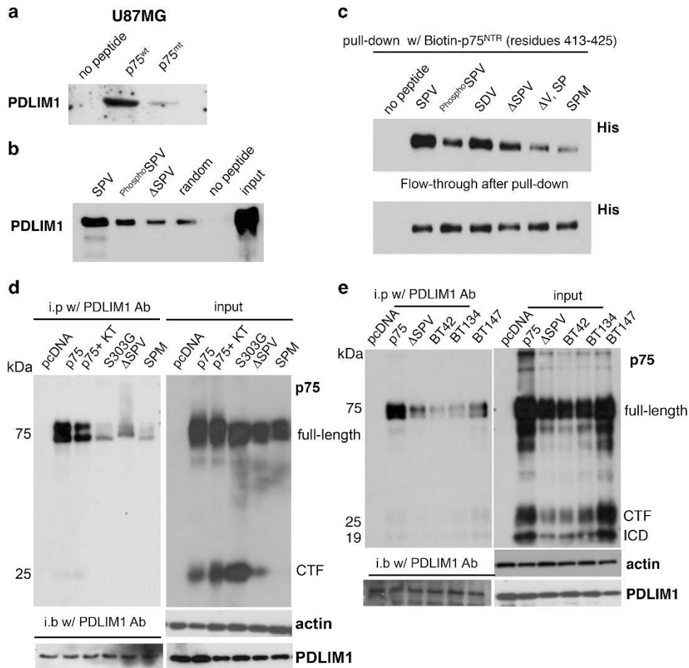
Figure 5. PDLIM1 associates with p75 NTR via the C-terminal PDZ-binding motif, an interaction regulated by phosphorylation of S425. (a) Using a biotinylated peptide to the C-terminus of either p75 NTR (p75 wt peptide, Biotin-N-LCSESTATSPV-COOH, residues 417-427) or a Valine deletion mutant of p75 NTR (p75 mt peptide, biotin-N-LCSESTATSP-COOH, residues 417-426) as affinity reagents, PDLIM1 was confirmed as a p75 NTR -interacting protein by western blot analysis. (b) To assess the physiological relevance of the phosphorylation of S425 within the PDZ-binding motif, biotin-labeled peptides corresponding to the p75 NTR wild-type C-terminal (SPV), the S425 phosphorylated C-terminal ( Phospho SPV) and the PDZ-binding motif deleted C-terminal ( \Delta SPV) were used as affinity reagents. PDLIM1 was shown to interact with maximum affinity to the wild-type unphosphorylated peptide. (c) Biotin-labeled p75 NTR peptides (SPV, Phospho SPV, \Delta SPV, \Delta V, SP and SPM) were incubated with His-tagged recombinant PDLIM1 protein, respectively. Pull-down assays were performed to determine the amount of PDLIM1 protein bound to each peptide. Flow-through shows unbound proteins after incubation. (d) Immunoprecipitation with PDLIM1 antibodies co-precipitated p75 NTR and PDLIM1 while the mutant alleles of p75 NTR (S303G, \Delta SPV and SPM) or p75 NTR cells treated with the PKA inhibitor KT5720 (KT; 200 nM) were severely compromised for PDLIM1 binding. (e) Interaction of PDLIM1 with p75 NTR was confirmed in patient-derived glioma stem cells/tumor-initiating cells (BT42, BT134, BT147) by immunoprecipitation using anti-PDLIM1. Input cell lysates were assessed by western blot analysis for expression of p75 NTR and PDLIM1.
