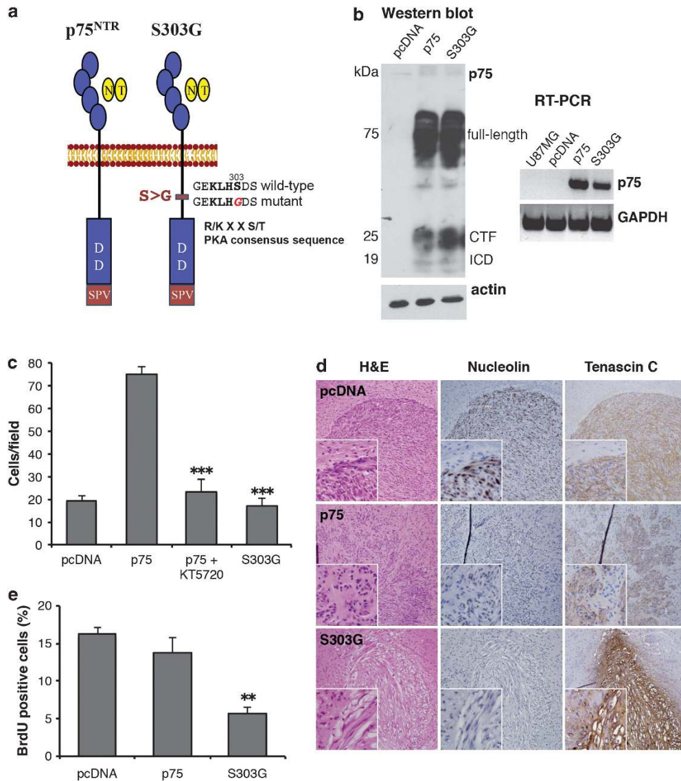
Figure 2. Mutation of the PKA phosphorylation site (S303G) abrogates p75 NTR -mediated invasion in vitro and in vivo . (a) Schematic diagram of wild-type and mutant p75 NTR constructs. p75 NTR has one putative PKA recognition consensus site (R/K X X S/T; KLHS) within the intracellular domain (ICD) of the protein. A PKA phosphorylation-defective mutant was generated by substitution of amino acid S303 by glycine (S303G). (b) U87MG glioma cells were stably transfected with pcDNA3.1 (pcDNA), pcDNA 3.1 containing wild-type p75 NTR (p75) or pcDNA 3.1 containing the S303G mutant of p75 NTR . RT-PCR and western blot confirm the expression of the wild-type and mutant receptors. RT-PCR analysis of GAPDH and western blot analysis of actin were included as loading controls. Western blot analysis detected the full-length p75 NTR , the 25-kDa C-terminal fragment (CTF) and the 19-kDa ICD of p75 NTR . (c) Invasion of S303G cells in collagen-coated transwell chambers was significantly decreased compared with wild-type p75 NTR -expressing cells (p75). Noninvasive U87pcDNA were used for comparison. Histogram shows the mean \pm s.e.m. from three independent experiments; asterisks (***) indicate P < 0.001 as compared with non-treated U87pcDNA (one-way ANOVA with the Neuman-Keuls post-test). (d) pcDNA, p75 and S303G cells ( 5 \times 10^4 cells) were implanted intracerebrally into SCID mice and allowed to grow for 28 days. The mice were killed, and paraffin brain sections were stained with Hematoxylin & Eosin (H&E) or antibodies against human nucleolin or tenascin-C (brown) to visualize the tumors. Sections were counterstained with hematoxylin (blue). (e) In vivo tumor proliferation was determined by injecting bromodeoxyuridine (BrdU) into tumor-bearing mice 24 h prior to killing of the mice. Frozen brain sections were stained with an antibody against BrdU and counterstained with toluidine blue to visualize the cell nucleus. Cells that had divided during the 24 h prior to killing of the mice stained positively for BrdU, and the percentage of BrdU-positive cells was counted. Histogram represents the percentage of BrdU-positive cells in five consecutive fields. Values shown are the mean \pm s.e.m. from five independent mice; asterisks (**) indicate P < 0.01 as compared with control U87pcDNA (one-way ANOVA with the Neuman-Keuls post-test).
