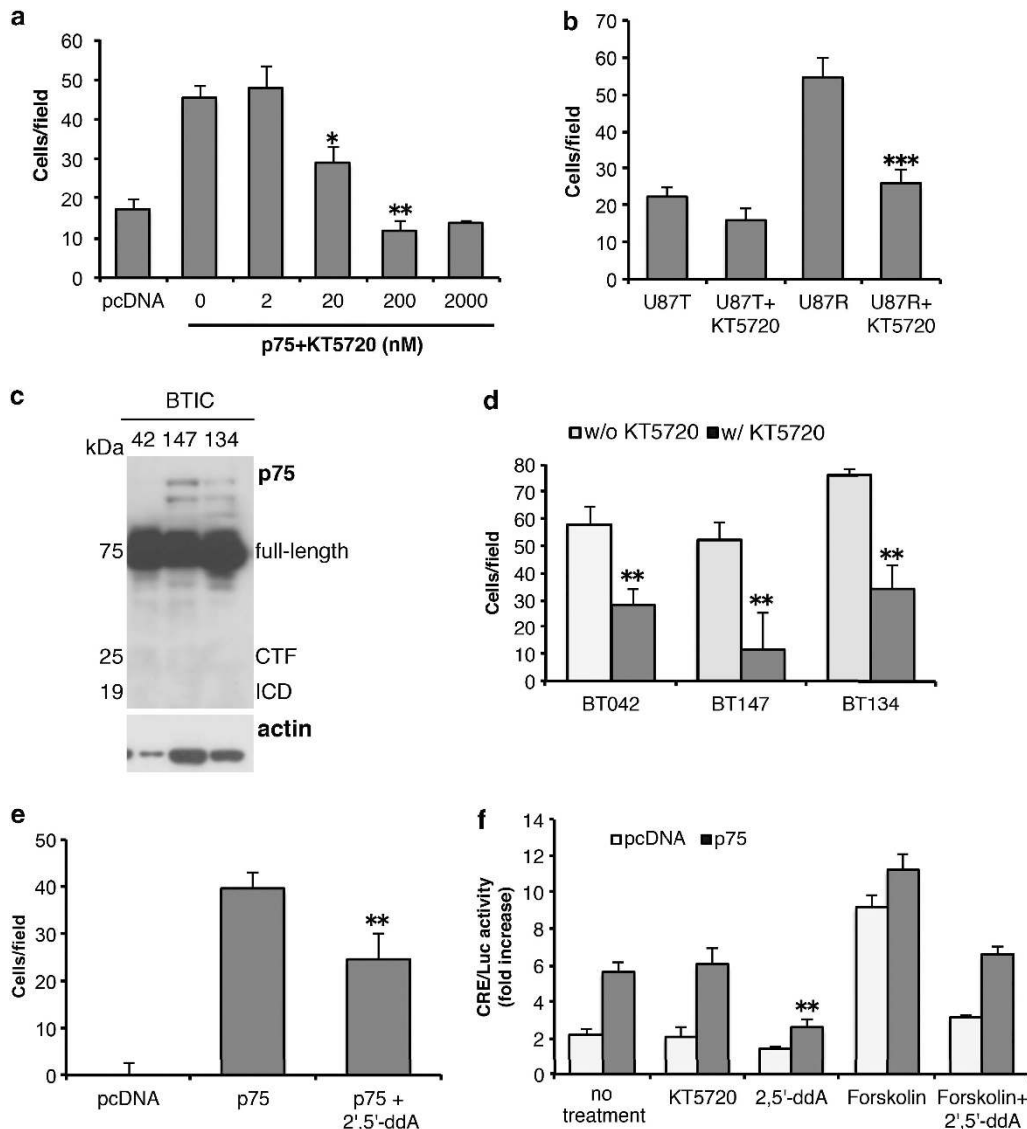
Figure 1. PKA inhibition significantly abrogated p75 NTR -induced glioma invasion. (a) Treatment with increasing concentrations of the PKA inhibitor KT5720 (KT) inhibited invasion of U87 cells expressing full-length p75 NTR (p75). Following pre-treatment with KT5720 for 1 h, the invasive ability of the U87 cells expressing full-length p75 NTR (p75) or empty vector (pcDNA; control) were determined using collagen-coated transwells. Similar results were observed in two independent experiments. Asterisk (*) indicate P < 0.05 and double asterisks (**) indicate P < 0.01 versus non-treated U87p75 cells (one-way ANOVA with the Newman-Keuls post-test). (b) Highly invasive U87R and noninvasive U87T cells were isolated by serial in vivo selection and assessed for their invasive ability in the absence or presence of KT5720 (200 nM). Asterisks (***) indicate P < 0.001 as compared with non-treated cells. (c) Western blot shows the expression of p75 NTR in patient-derived glioma cells BT042, BT147 and BT134. (d) Histogram shows that the invasion of the patient-derived glioma cells (BTIC) in the presence of fetal bovine serum was suppressed by KT5720 (200 nM). Asterisks (**) indicate P < 0.01 as compared with the corresponding non-treated BTIC. (e) p75 NTR -mediated glioma invasion is dependent on cAMP. U87pcDNA or p75 cells were treated for 1 h with an adenylyl cyclase inhibitor (2', 5'-dideoxyadenosine(2', 5'-dda)) and invasion assays (described above) were performed. Asterisk (**) indicate P < 0.01 versus non-treated U87p75 cells. (f) U87p75 NTR treated with the PKA inhibitor KT5720 (1 h, 200 nM), 2', 5'-dda (1 h, 30 \mu M) or the adenylyl cyclase activator forskolin (1 \mu M) in the presence or absence of 2', 5'-dda were assessed for cAMP activity using a CRE-luciferase reporter construct. Histogram shows the fold increases in luciferase activity as compared with vehicle-treated cells. Asterisk (**) indicate P < 0.01 versus non-treated U87p75 cells. Data represent the mean \pm s.e.m. of triplicates, representative of at least three independent experiments.
