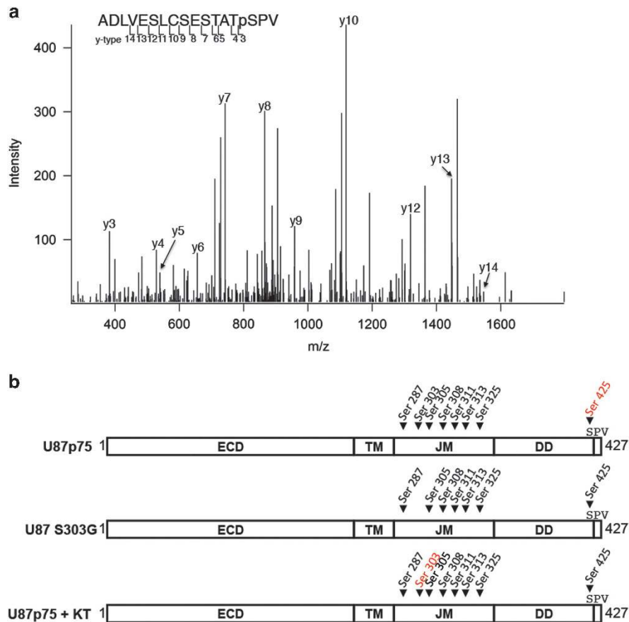
Figure 3. PKA regulates the phosphorylation of S425 within the p75 NTR -PDZ binding motif. p75 NTR (U87p75), mutant S303G p75 NTR or cells expressing p75 NTR that were treated with the PKA inhibitor KT5720 (200 nM) were lysed, immunoprecipitated with anti-p75 NTR , run on 10% sodium dodecyl sulfate–polyacrylamide gel electrophoresis and proteins were visualized by silver stain. Protein bands representing p75 NTR were removed from the gel and in-gel trypsin digestion was performed. Digested peptides and phosphorylated serine residues were identified using nano-liquid chromatography–tandem mass spectrometry (LC/MS/MS) on a LTQ Orbitrap velos (Thermo Scientific; Southern Alberta Mass Spectrometry Center). (a) Modification and peptide search were performed with Mascot software v2.3. The MS/MS spectrum for the phospho-peptide ADLVESLCSESTAT(pS)PV, with annotated b and y ions, is shown. Phosphorylation at serine -1 is indicated by presence of y3 ion (+80Da for the mass of the phosphate group). (b) Shown is a schematic representation of p75 NTR indicating serine phosphorylated residues (black text) within the intracellular domain of p75 NTR isolated from U87 cells expressing wild-type p75 NTR (U87p75), mutant S303G p75 NTR or cells expressing p75 NTR that were treated with the PKA inhibitor KT5720 (200 nM). Red text indicates unphosphorylated serine residues.
