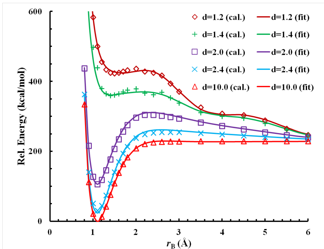
Figure S5. Dissociation curves for N_2 + N_2 : comparison of the global fit to the values obtained with the CASPT2 method for the Z-shaped set with one N_2 fixed to its equilibrium distance.
