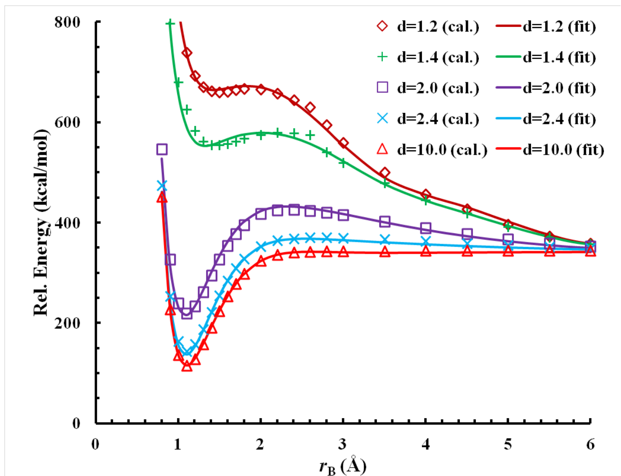
Figure S6. Dissociation curves for N_2 + N_2 : comparison of the global fit to the values obtained with the CASPT2 method for the Z-shaped set with one N_2 fixed to 0.898 \text{ \AA} .
