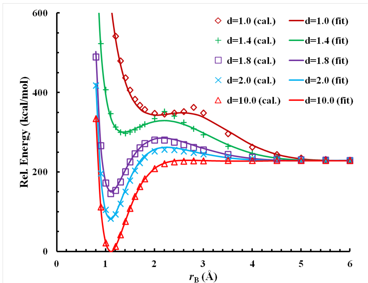
Figure S2. Dissociation curves for N_2 + N_2 : comparison of the global fit to the values obtained with the CASPT2 method for the bent H-shaped set with one N_2 fixed to its equilibrium distance; r_B is dissociating.
