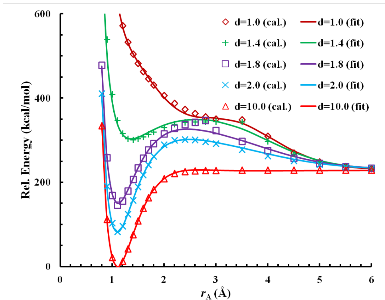
Figure S1. Dissociation curves for N_2 + N_2 : comparison of the global fit to the values obtained with the CASPT2 method for the bent H-shaped set with one N_2 fixed to its equilibrium distance; r_A is dissociating.
