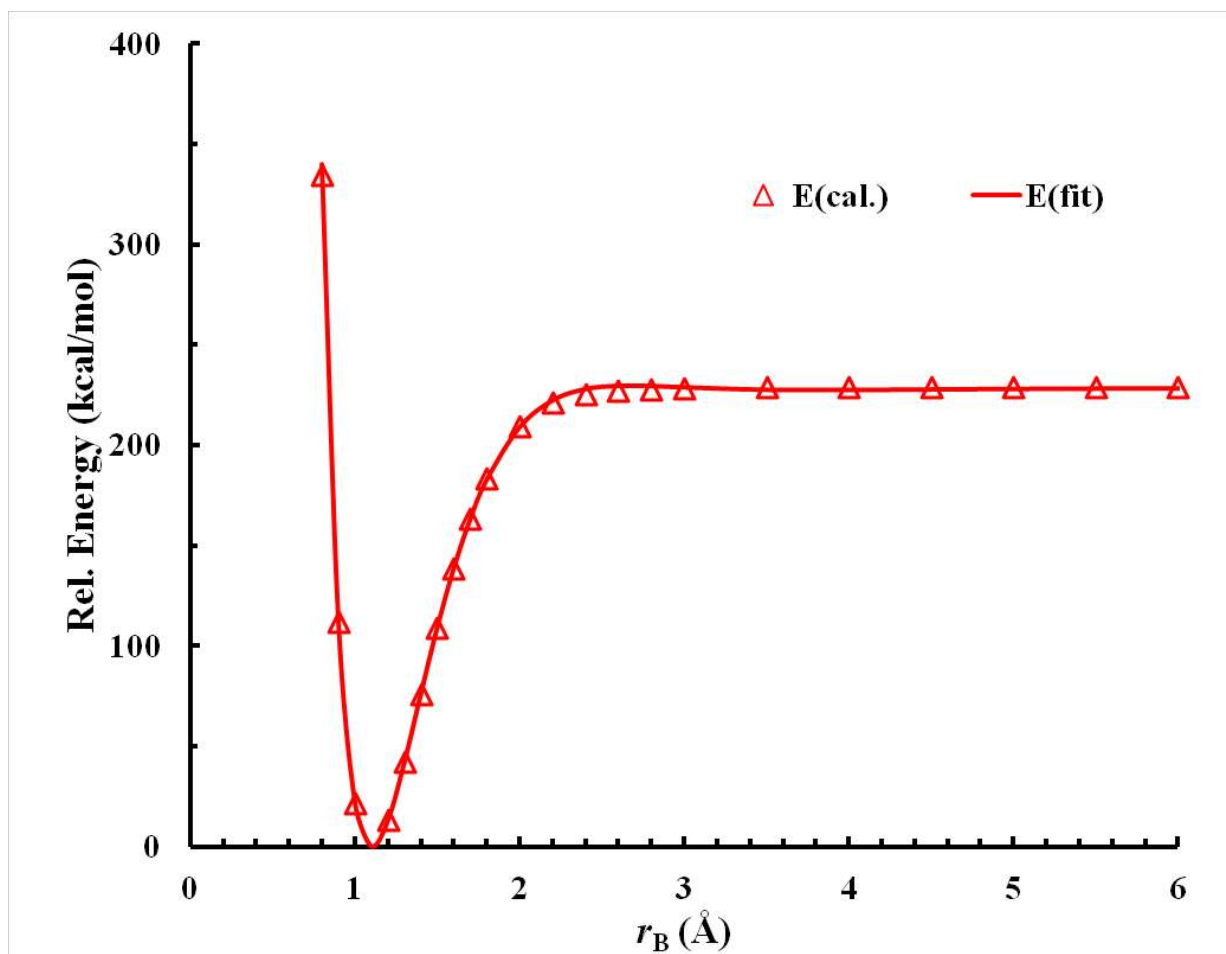
Figure S8. Dissociation curves for N_2 : comparison of the fit to the values obtained with the CASPT2 method.
