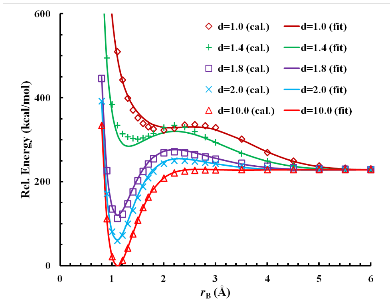
Figure S4. Dissociation curves for N_2 + N_2 : comparison of the global fit to the values obtained with the CASPT2 method for the bent X-shaped set with one N_2 fixed to its equilibrium distance.
