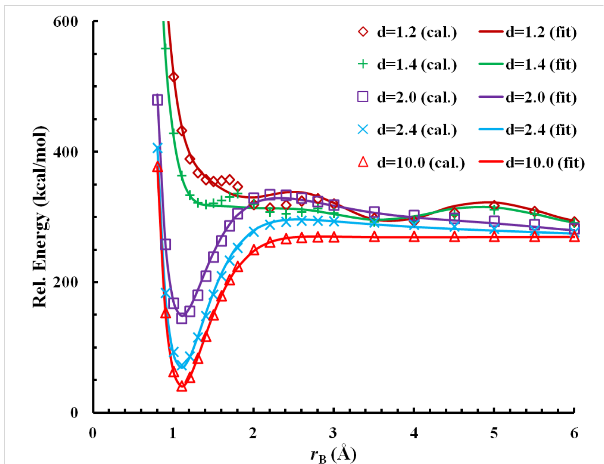
Figure S7. Dissociation curves for N_2 + N_2 : comparison of the global fit to the values obtained with the CASPT2 method for the Z-shaped set with one N_2 fixed to 1.298 \text{ \AA} .
