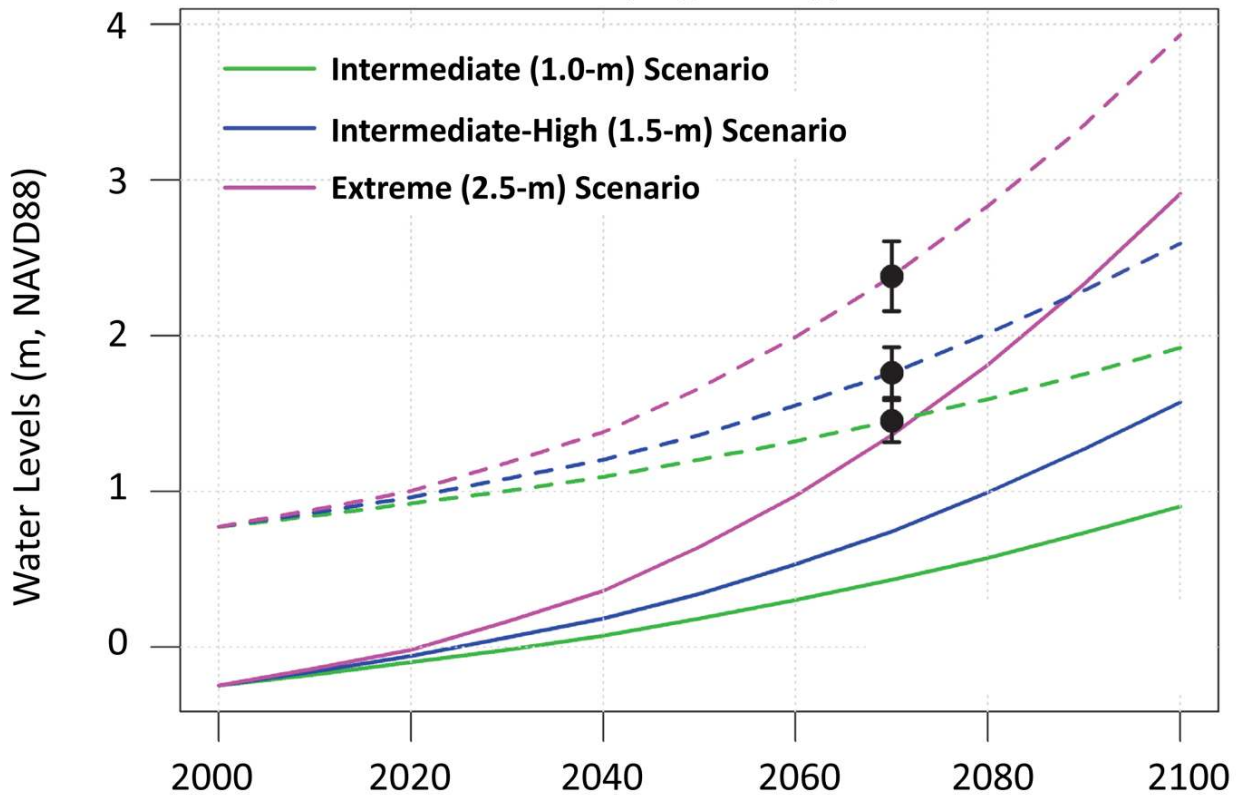
Figure 17. RSL under the Intermediate (1-m), Intermediate-High (1.5-m), and Extreme (2.5-m) GMSL rise scenarios (solid curves) for Florida Keys region, showing how the water level height with a 1% annual chance of occurring (dashed lines) and 95% confidence intervals (black error bars) estimated for year 2070 from hourly water levels at the NOAA Key West tide gauge changes in magnitude under each scenario. All curves have been expressed in terms of the geodetic datum NAVD88 using the tidal datums at Key West.
