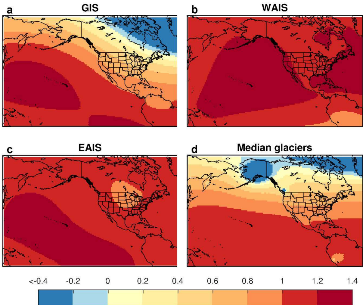
Figure 7. Ratio of RSL to GMSL change for mass loss from specific land-ice sources; these constitute the static-equilibrium fingerprints of the source. a) Greenland ice sheet (GIS), b) West Antarctic ice sheet (WAIS), c) East Antarctic ice sheet (EAIS) and d) the median of 18 mountain glaciers after Kopp et al. 2014, 2015. Values more than (less than) 1 indicate RSL rise higher (lower) than GMSL rise.
