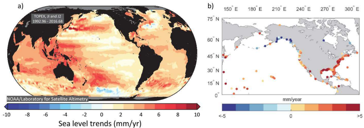
Figure 4. a) Sea level change rates from 1992-2016 from TOPEX/Poseidon, Jason-1 and Jason-2 ( www.star.nesdis.noaa.gov/sod/Isa/SeaLevelRise ) and b) relative sea level trends based upon full record (>30-year period of record in all cases) measured and published for NOAA tide gauges through 2015 ( tidesandcurrents.noaa.gov/sltrends ).
