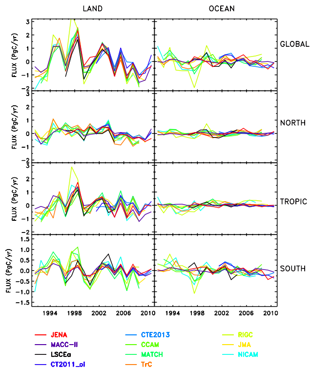
Fig. 6. Annual mean anomalies of the individual participating inversion posterior flux estimates. Shown here are the fossil-fuel-corrected natural land (first column) and natural ocean (second column) carbon exchange for the same regions as Fig. 4: global, north ( > 25^\circ N), tropics ( 25^\circ S– 25^\circ N) and south ( < 25^\circ S).
